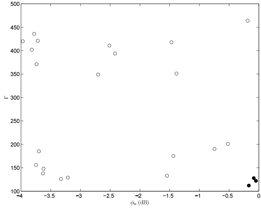
Figure 6: State space realization solution set showing \phi_u against \Gamma . 5th-order controllers are marked ●, and 7th-order controllers are marked ○.
