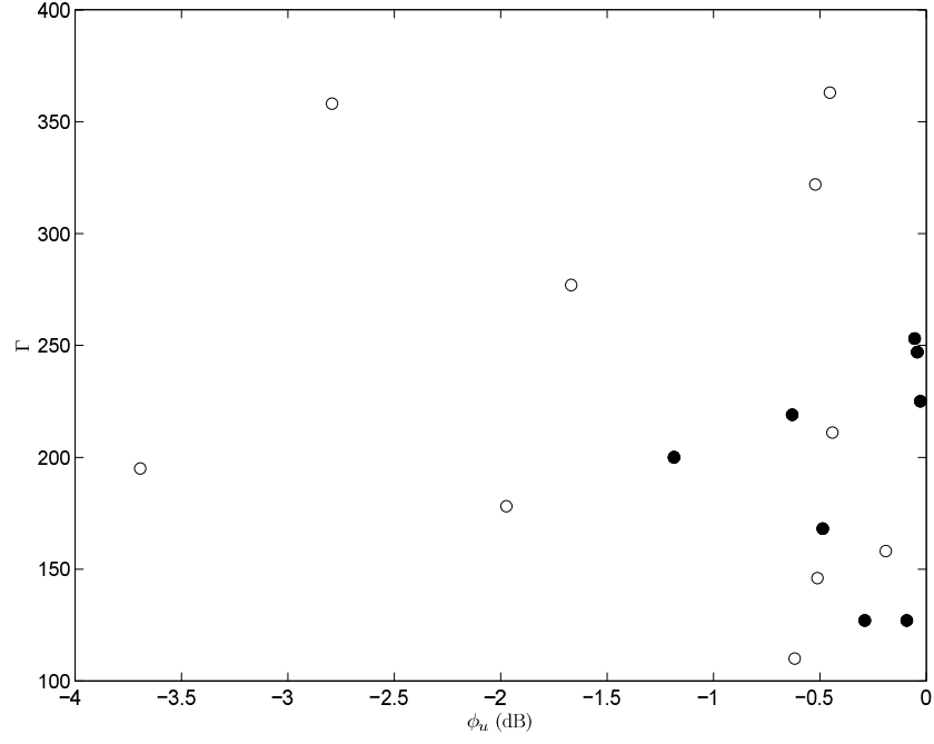
Figure 9: Parallel and cascade realization solution set showing \phi_u against \Gamma . 5th-order controllers are marked ●, and 7th-order controllers are marked ○.
