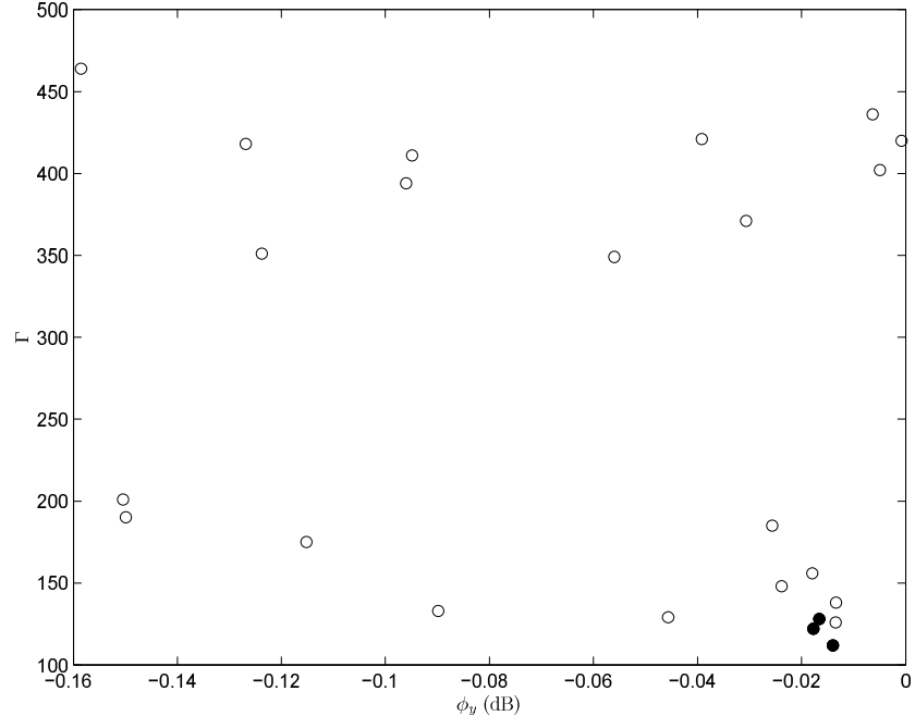
Figure 5: State space realization solution set showing \phi_y against \Gamma . 5th-order controllers are marked ●, and 7th-order controllers are marked ○.
