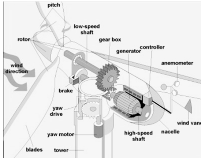
Figure 5– Wind turbine components (source: NREL).
