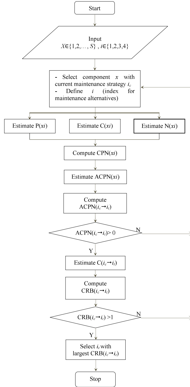
Figure 4— Cost-risk-benefit analysis for maintenance strategy selection/updating.
