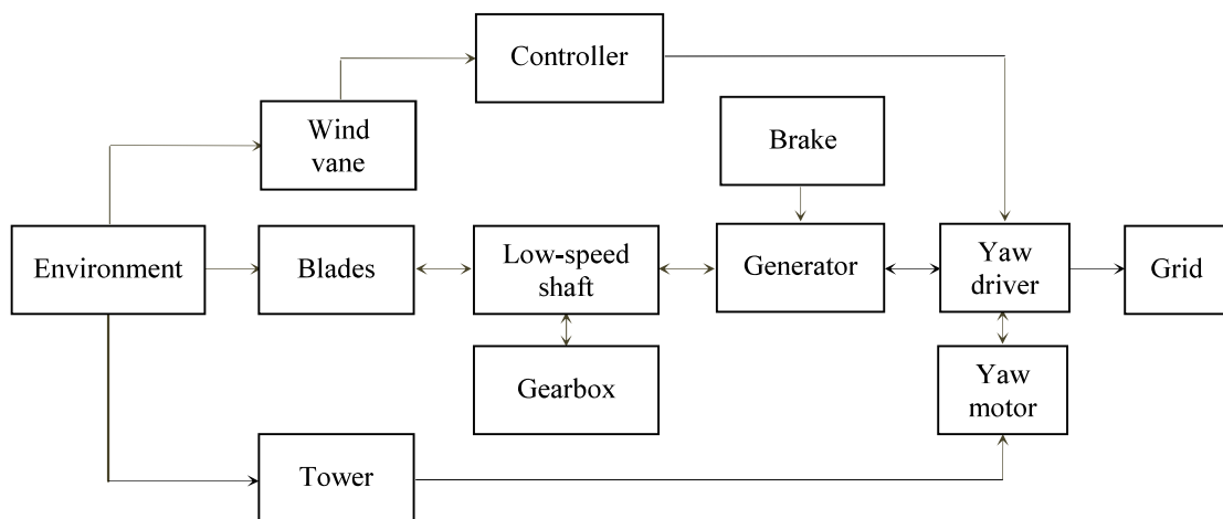
Figure 6– A dependency diagram for wind turbine components ( \rightarrow : dependence ; \leftrightarrow : interdependence).
