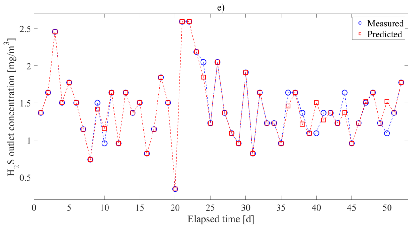
Figure 2. Predictions of H_2S outlet concentrations from the MBBR using (a) ANN, (b) multi-task ANN, (c) SVM, (d) RF, and (e) LSBoost models.
