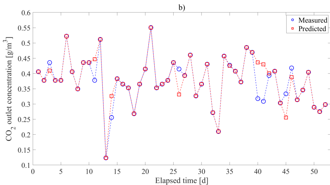
Figure 6. LSBoost+LSBoost approach for predicting (a) \text{H}_2\text{S} and (b) \text{CO}_2 outlet concentrations from the MBBR+aPBR integrated system.
