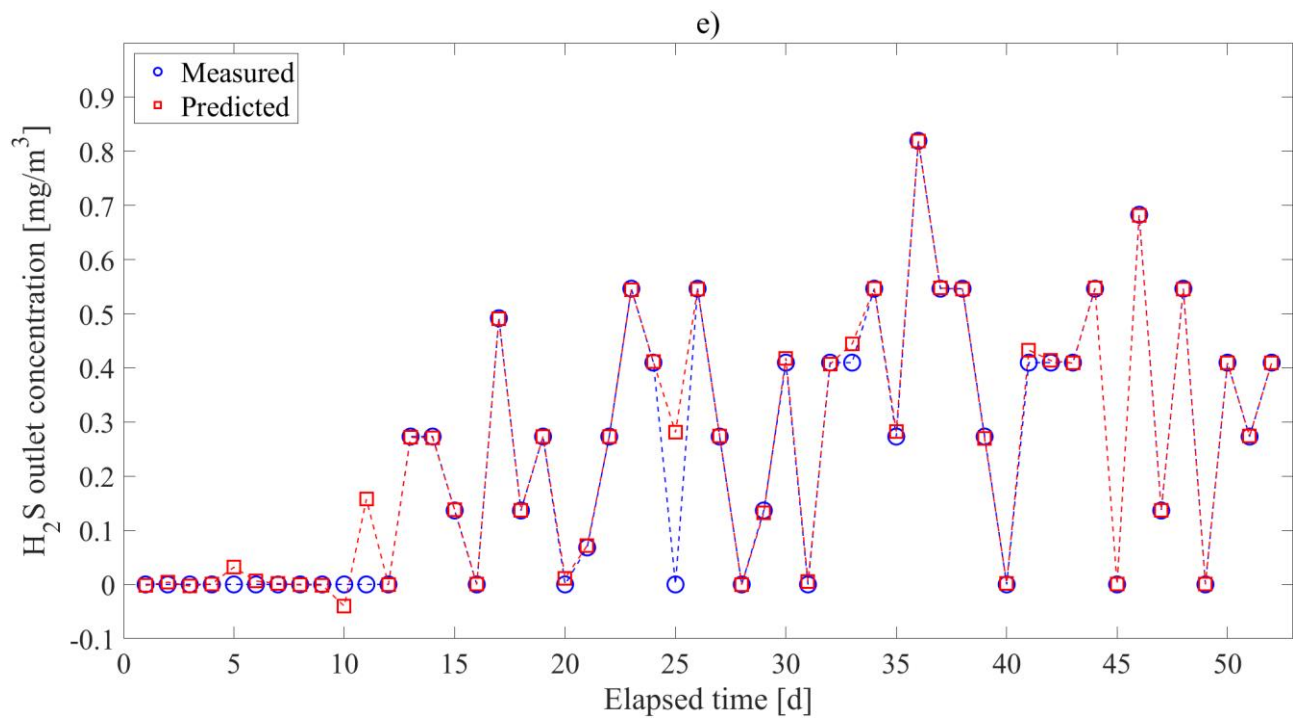
Figure 4. Predictions of H_2S outlet concentrations from the aPBR using (a) ANN, (b) multi-task ANN, (c) SVM, (d) RF, and (e) LSBoost models.
