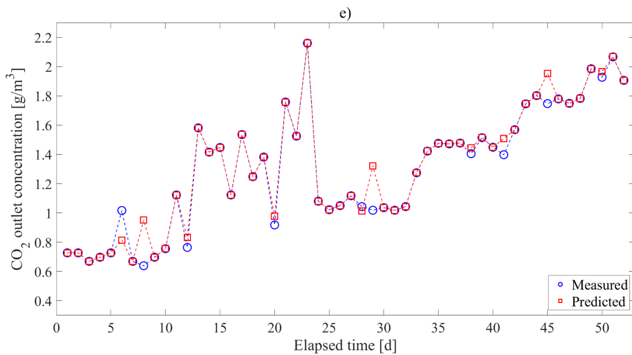
Figure 3. Predictions of CO 2 outlet concentrations from the MBBR using (a) ANN, (b) multi-task ANN, (c) SVM, (d) RF, and (e) LSBoost models.
