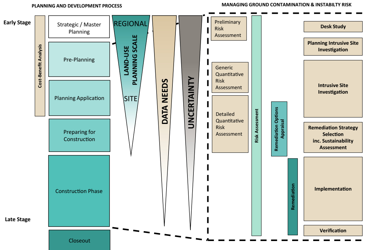
Fig. 1. The typical planning and land development process for brownfield sites indicating the relationship between steps within each domain showing how scale, data and uncertainty reduce over time. BGS © UKRI 2021 and Cranfield University © 2021.
