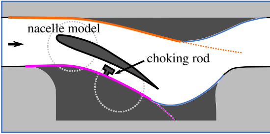
Figure 7: Schematic generation of the wind tunnel geometry for a) end-of-runway windmilling and b) diversion windmilling: i. 3D RANS simulations of the entire nacelle; ii. streamlines from a slice through the vertical plane; iii. the wind tunnel geometry with wall contours defined by extracted streamlines.
