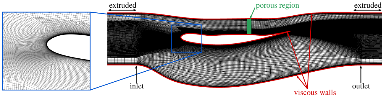
Figure 8: Mesh for 2D computations of the wind tunnel flow path.
