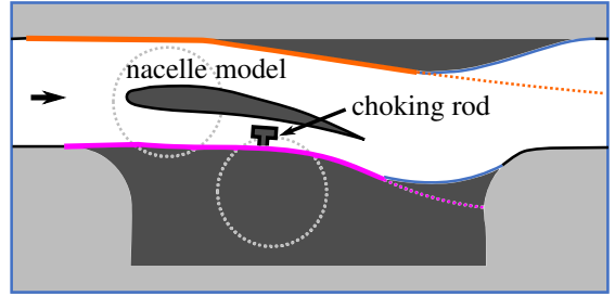
Figure 7: Schematic generation of the wind tunnel geometry for a) end-of-runway windmilling and b) diversion windmilling: i. 3D RANS simulations of the entire nacelle; ii. streamlines from a slice through the vertical plane; iii. the wind tunnel geometry with wall contours defined by extracted streamlines.
