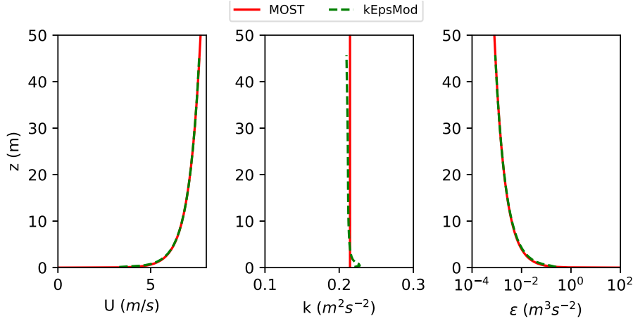
Fig. 7 Comparing ABL profiles at outlet boundary of Burro9 simulation using modified k - \epsilon model (kEpsMod) and MOST inlet profiles (MOST)
