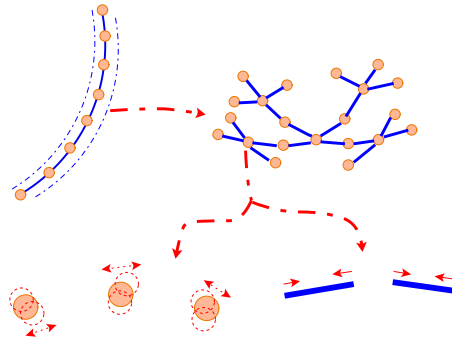
Figure 1: Metastructure concept: many linked elements are actively controlled to give the resulting structure its desired geometry.
