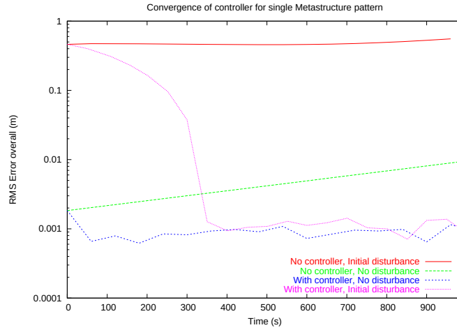
Figure 3: Controller performance for an initially disturbed and undisturbed state for the reference structure. The disturbed state is an initial inclination of 15^\circ in and out of plane. The Y axis represents the Root Mean Squared Position Error overall (in m).
