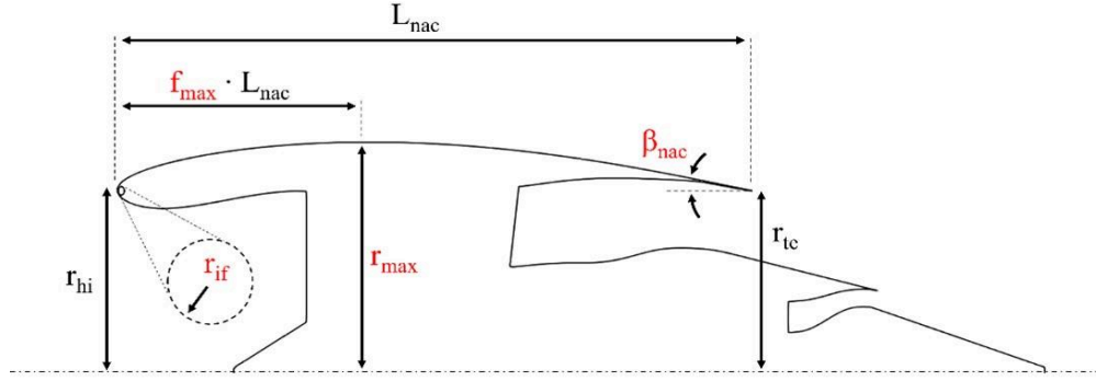
Figure 1: 2D axisymmetric nacelle parameterisation. Parameters marked in red are floated in the optimisation process.
