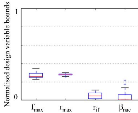
Figure 5: Optimal design space obtained for the CFD-in-the-loop optimisation.
