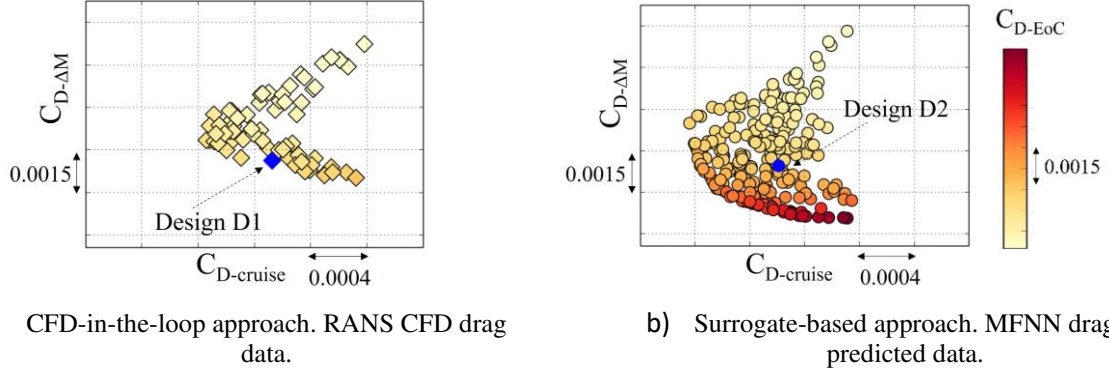
Figure 8: Pareto fronts and down selected designs from the optimisations using the CFD-in-the-loop and the surrogate-based approaches.
