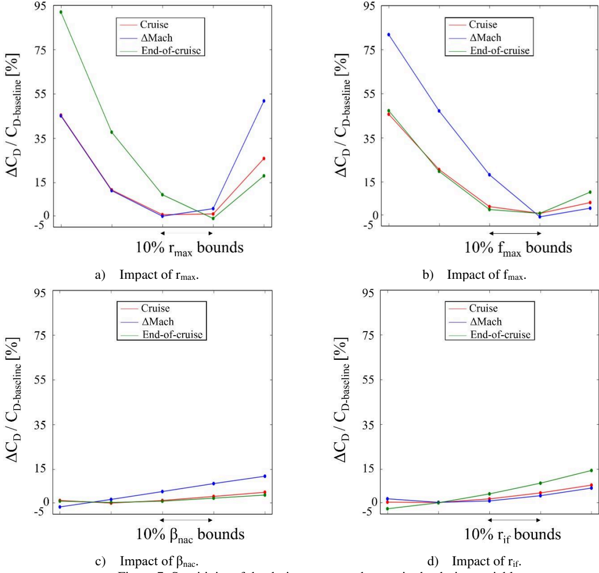
Figure 7: Sensitivity of the design space to changes in the design variables.
