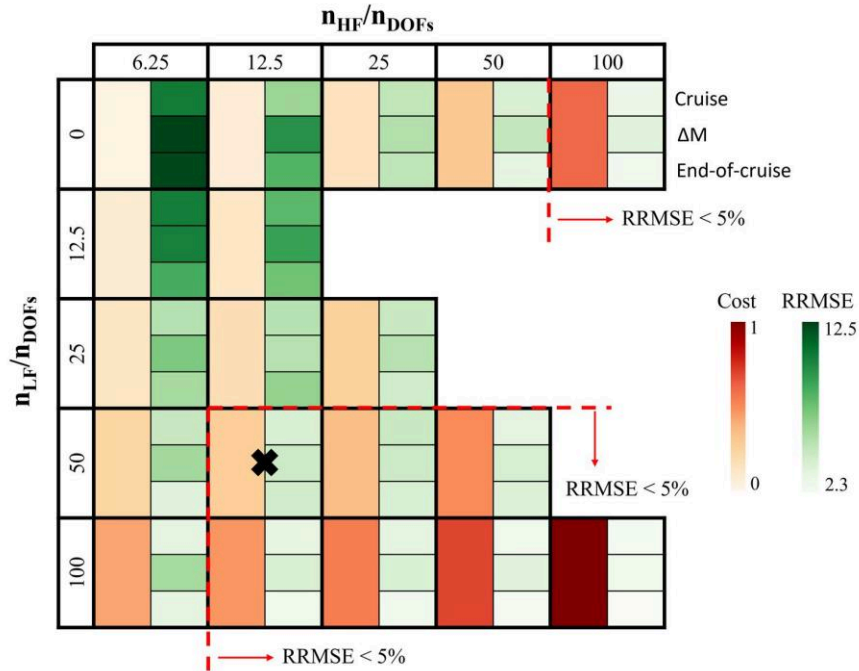
a) Impact of the number of low- and high-fidelity samples on the computational cost and RRMSE of the surrogate model. Black cross: optimum trade-off combination between cost and model error.
