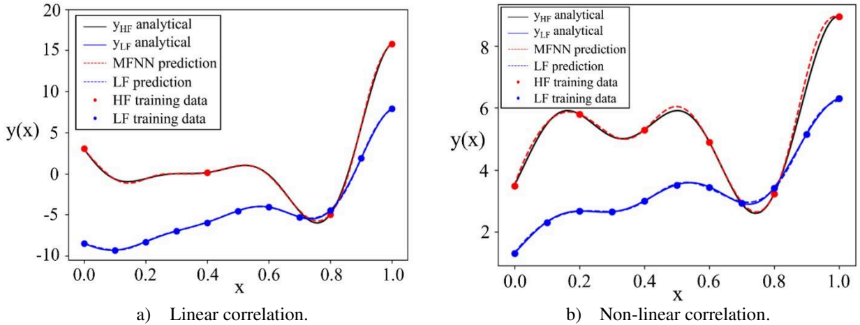
Figure 3: MFNN prediction for the one-dimensional benchmark function.
