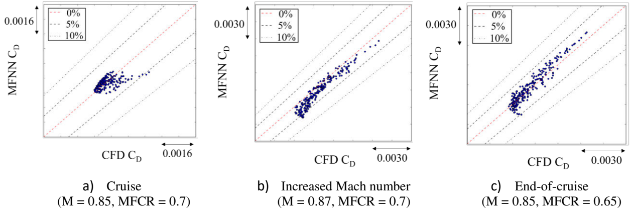
Figure 9: Surrogate model performance in the optimal design space using the designs in the Pareto front obtained in the MFNN-based optimisation.
