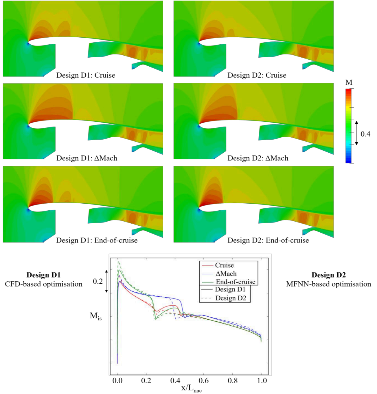
Figure 10: Mach number distributions for the down selected designs using the CFD-in-the-loop and surrogate-based optimisation approaches.
