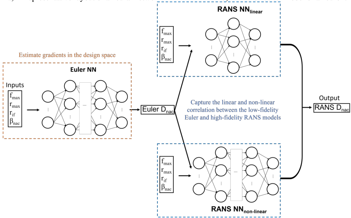
c) Architecture of the MFNN method.
