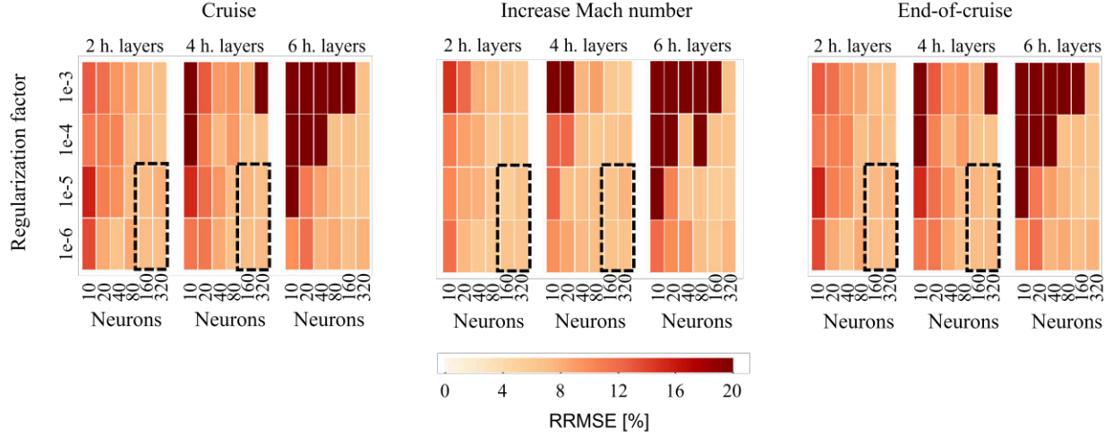
Figure 4: Hyperparameter sensitivity analysis of the low-fidelity network for different operating conditions. ReLu activation function. Training dataset of n_{LF}/n_{DOFs} = 100 .
