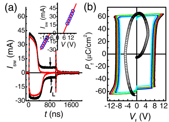
FIG. 4. (Color online) (a) Positive/negative domain switching current transient for BFO with an electrode area of 8.35 \times 10^{-5} \text{ cm}^2 at V = \pm 12 V and pulse width of 1000 ns before (a solid line) and after (a dashed line) leakage current deduction, where the inset shows the voltage dependence of domain switching current fitted by two solid lines. (b) The transferred P - V hysteresis loops from domain switching currents, where the opened symbols show the measurement from a Radiant tester at 50 kHz.
