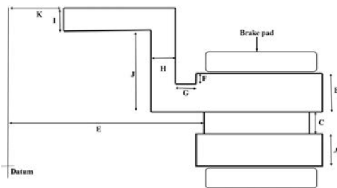
Figure 1. Brake disc diagram showing design features
