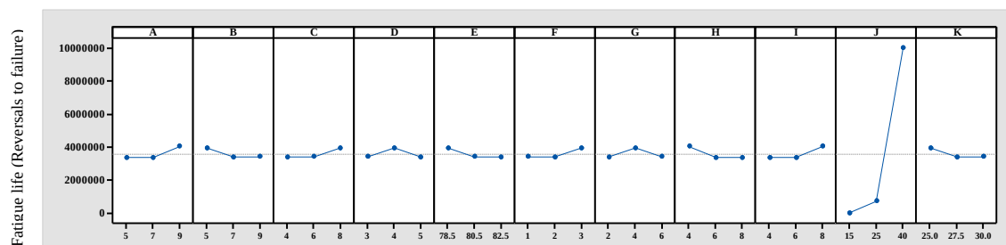
Figure 3. Effect diagram for sensitivity of fatigue at hub mounting surface corner
