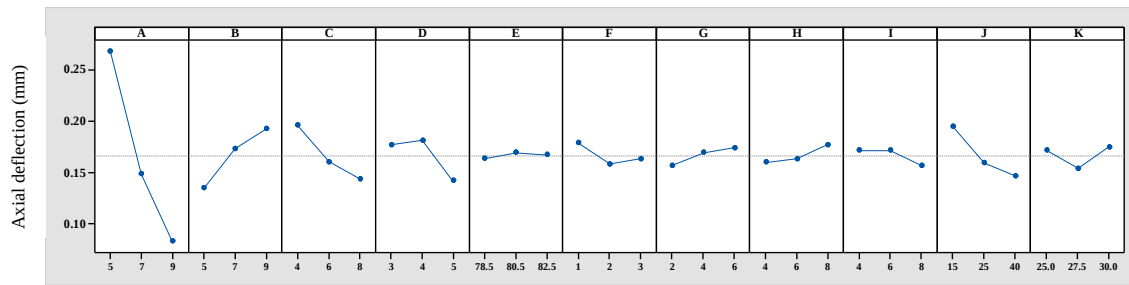
Figure 4. Effect diagram for sensitivity of axial deflection
