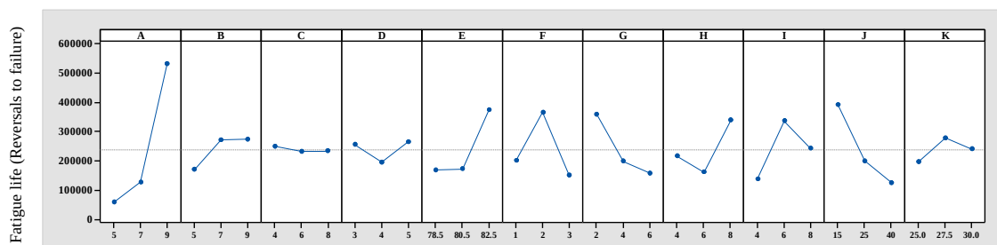
Figure 2. Effect diagram for sensitivity of fatigue at hat-friction plate corner
