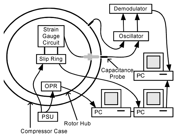
Fig. 3. On-Rotor Experiment Set-Up
