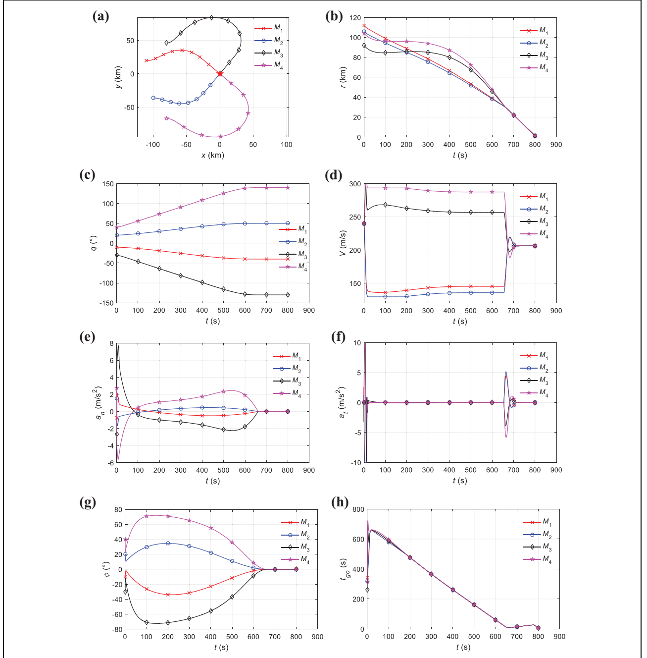
Figure 4. Numerical simulation results for case I: (a) missiles-target trajectories in horizontal plane, (b) missiles-target relative distances, (c) missiles' LOS angles, (d) missiles' velocities, (e) normal accelerations achieved by autopilot, (f) tangential accelerations achieved by autopilot, (g) missiles' lead angles, and (h) time-to-go estimates relative to virtual targets. LOS: line-of-sight.
