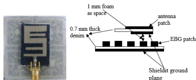
Fig. 3. Configuration of antenna with EBG structure.
