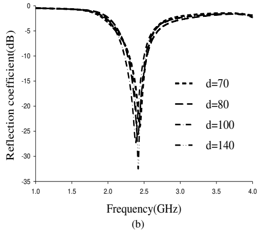
Fig.7. Reflection coefficient (S11) of antenna with EBG structure for different bending diameters (in mm) at the (a) y-axis and (b) x-axis
