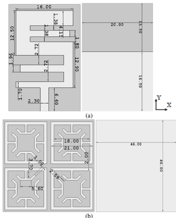
Fig. 2. EBG characteristics based on reflection phase and suspended line.
