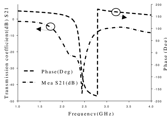
Fig. 2. EBG characteristics based on reflection phase and suspended line.
