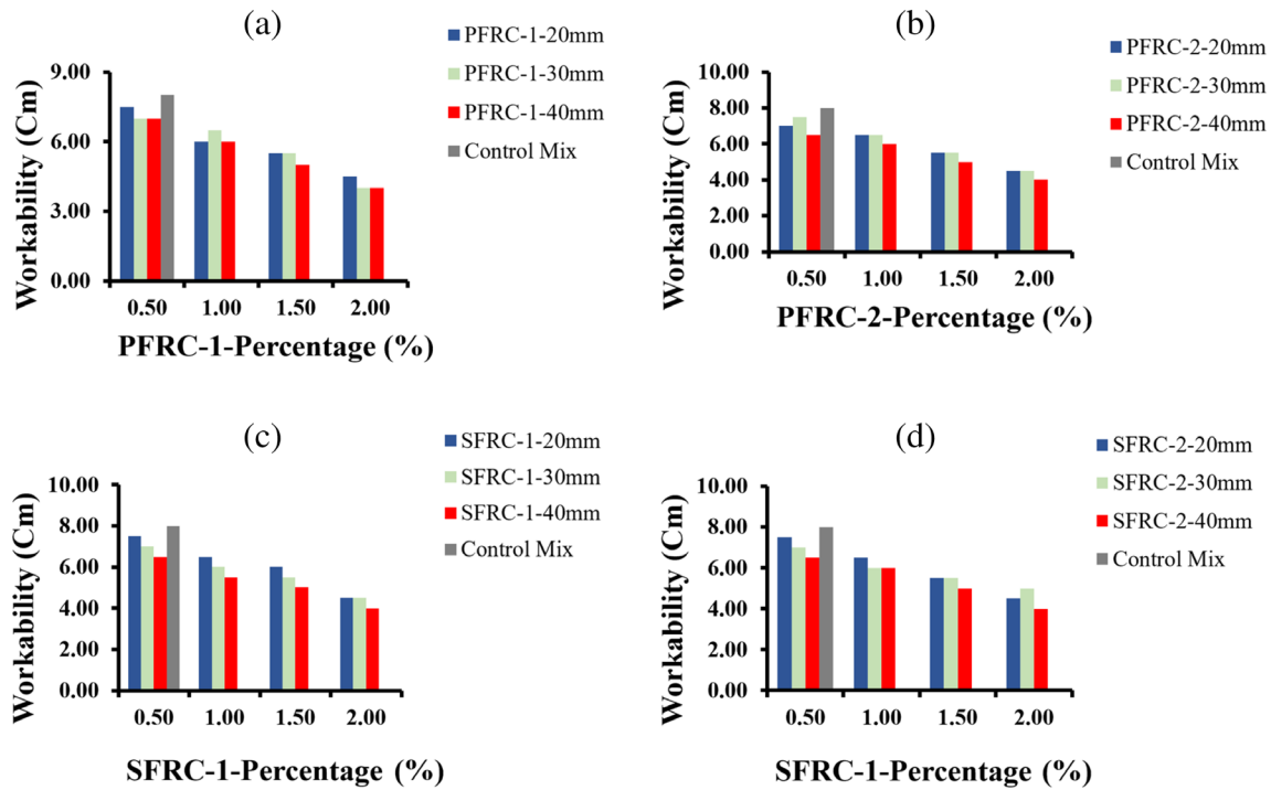
FIGURE 7 Impact of different types of fiber on concrete workability.
