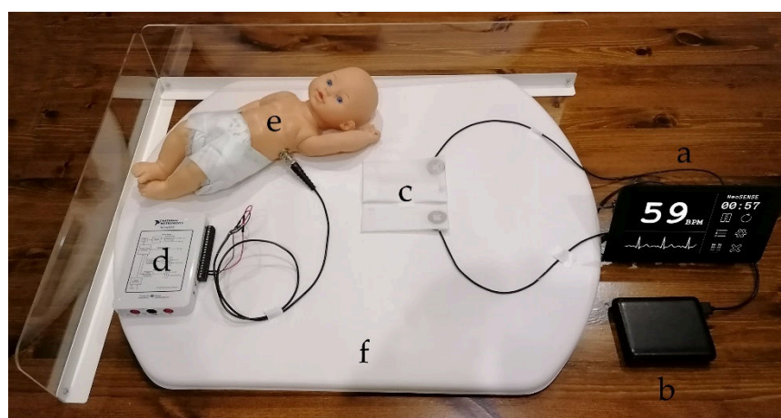
Figure 10. Photograph of prototype system hardware in neonate simulation environment: (a) front end and GUI (Dimensions 195 × 100 × 90mm); (b) USB 5V power bank; (c) EPS sensors and textile based electrodes; (d) digital to analogue converter for test signal generation; (e) neonate mannequin with internal antenna; (f) commercial delivery room mattress.
