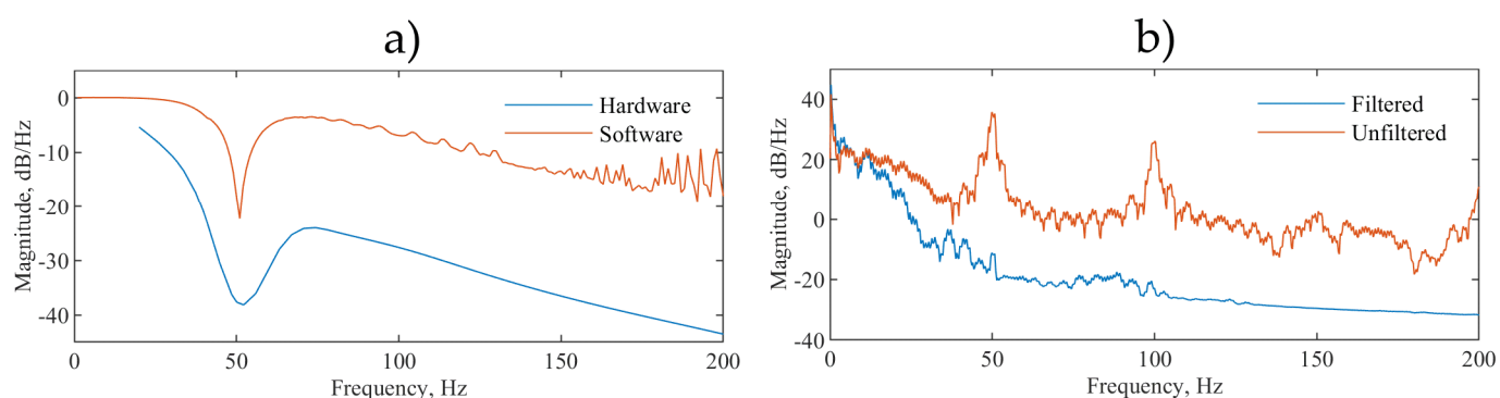
Figure 7. (a) Frequency response analysis of hardware and software stages, (b) power spectral density showing the combined effect of hardware and software filtering on a noisy test ECG signal injected directly into the front end.
