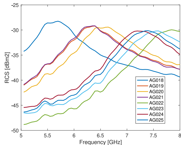
FIGURE 7 RCS of the aluminised glass dipoles as a function of frequency in the bandwidth between 5 and 8 GHz.
