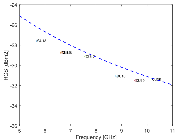
FIGURE 6 Peak RCS for each copper wire dipole as a function of the frequency at which the peak occurs. The blue dashed curve indicates the expected theoretical RCS as a function of frequency.
