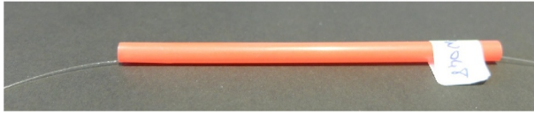
FIGURE 2 Dipole on a nylon monofilament protected in a length of drinking straw.
