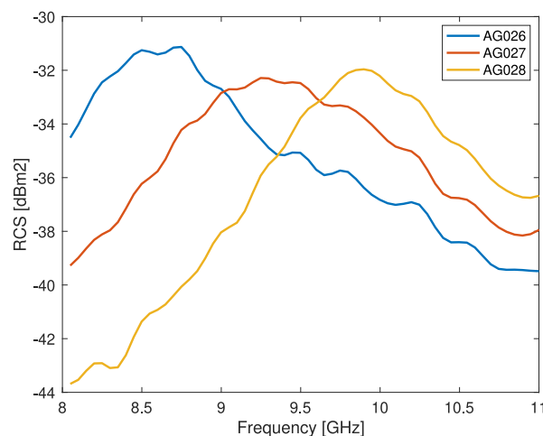
FIGURE 8 RCS of the aluminised glass dipoles as a function of frequency in the bandwidth between 8 and 11 GHz.
