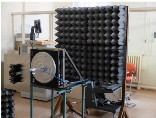
FIGURE 1 Measurement setup.
