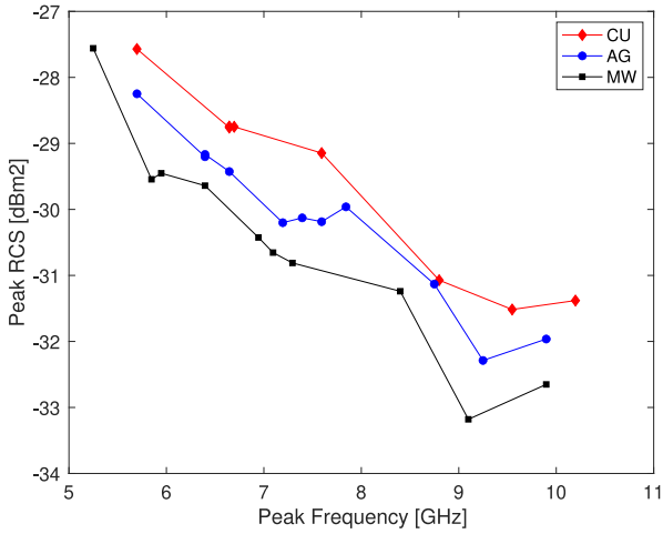
FIGURE 13 Comparisons of dipole RCS values.
