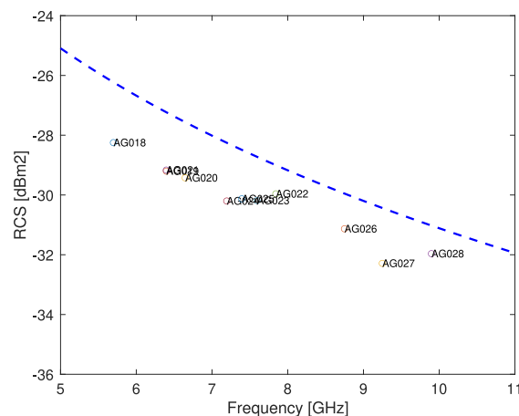
FIGURE 9 Peak RCS for each aluminised glass dipole as a function of the frequency at which the peak occurs.
