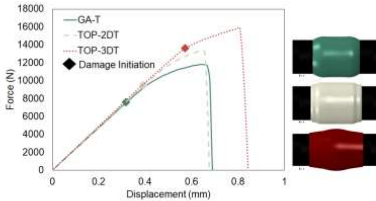
Figure 15 force-displacement graph for the optimized joints (3D tension)
