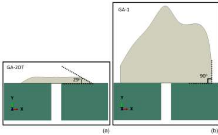
Figure 8 GA optimization process joints (a) Maximum SRF design (b) Maximum strength design
