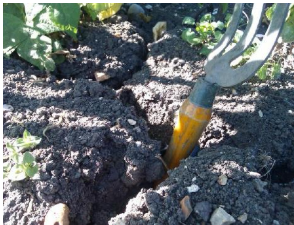
Figure 54 - Soil cracking in shrinkable soil in Cheddington (in the Anglian Water Region) Photo: I Truckell
