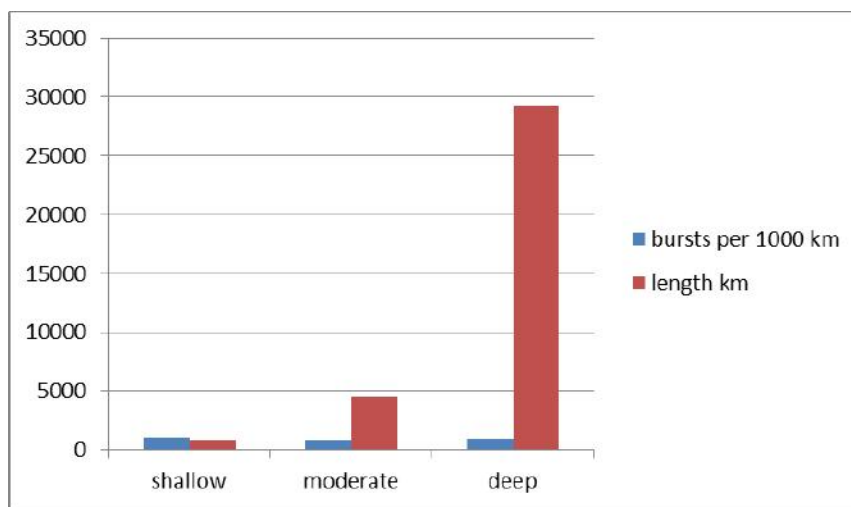
Figure 31 - Comparison of burst rates in soils of different depths.
