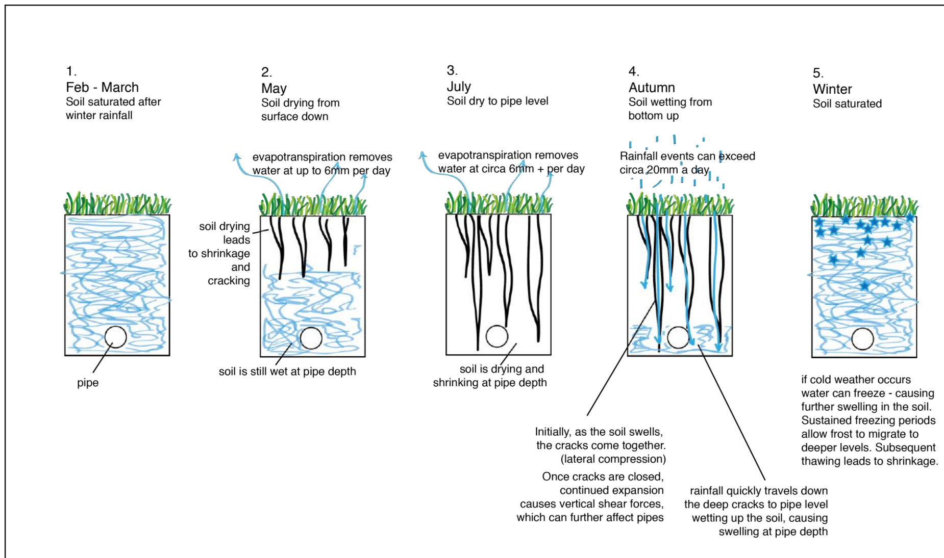
Figure 61 - The seasonal processes effecting soil movement and pipe failure
