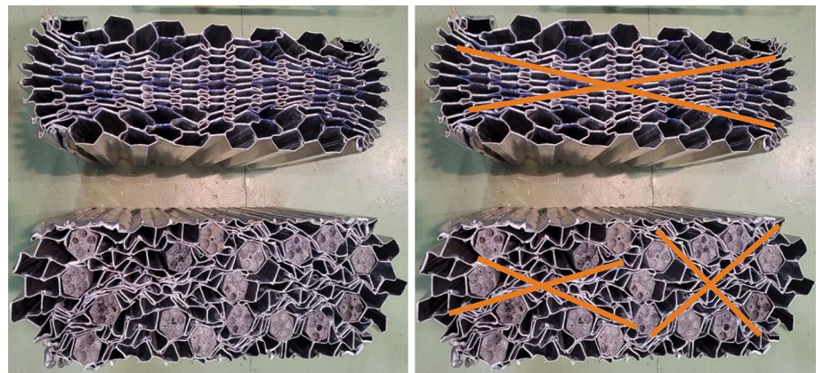
Fig. 8 Top view and deformation pattern of empty and foam-filled specimens after the L-direction quasi-static tests
