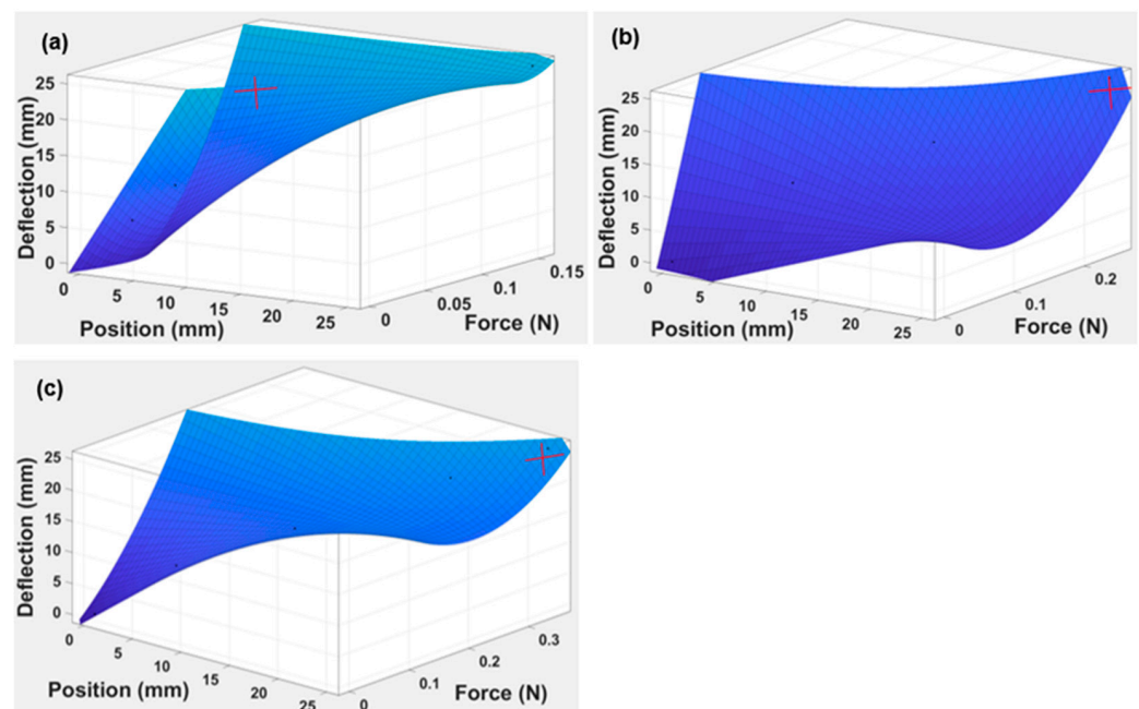
Figure 10. The 3D gradient graph illustrates the correlation between applied load (N), position (mm), and deflection (mm) for three different thicknesses of the TPE “cross” capsule. These thicknesses were (a) 1 mm, (b) 2 mm, and (c) 3 mm.
