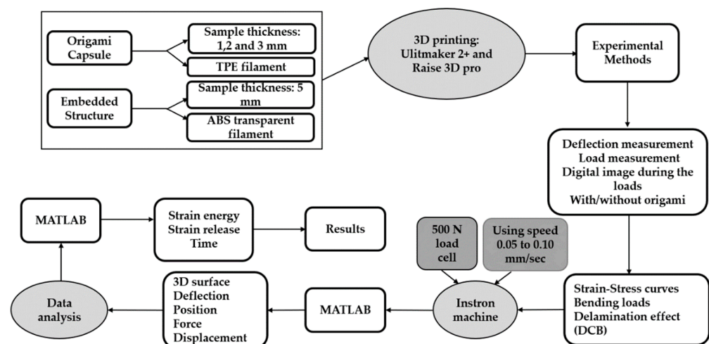
Figure 1. Methodology diagram.
