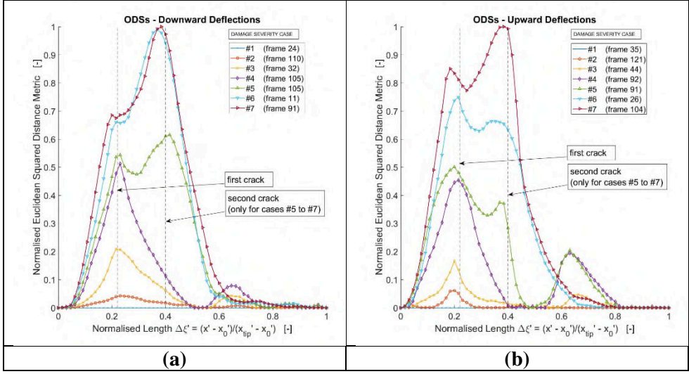
Fig 9. Normalised Euclidean Square Distance (ESD), as a metric of difference between damaged and undamaged ODSs, considering downward (a) and upward (b) deflections. The two metrics peak in correspondence of the cut cross-sections.
