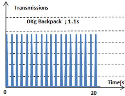
Figure 6. Time gap between transmissions for BAN.
