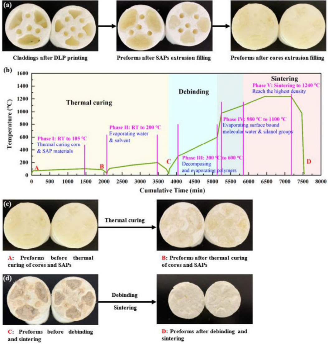
Fig. 6. Post-printing processing: (a) fibre preforms completed by extrusion filling of cores and SAPs in the printed cladding; (b) thermal processing of the completed fibre preforms; (c) the completed fibre preforms before (A in (b)) and after (B) thermal curing; (d) the cured fibre preforms before (C) and after (D) debinding and sintering.
