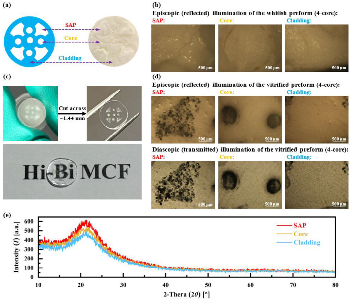
Fig. 7. Characterization of the resulting fibre preforms: (a) structural and physical diagrams of the 4-core whitish fibre preform (D in Fig. 6(d)); (b) polarized microscope images of the whitish fibre preform in (a) under episcopic illumination; (c) physical diagrams of the 4-core vitrified fibre preform; (d) polarized microscope images of the vitrified fibre preform under episcopic (top) and diascope (bottom) illumination; (e) XRD patterns of the vitrified fibre preforms. All results include the three parts of the fibre preforms: SAP, core, and cladding.
