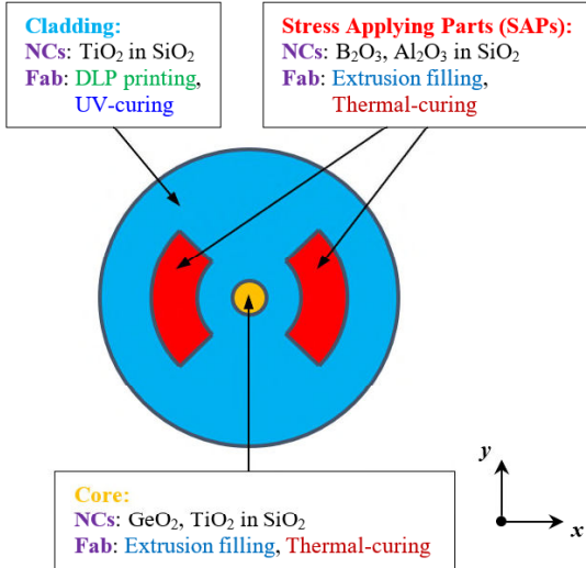
Fig. 1. Proposed Hi-Bi preform scheme using dual-curing resins incorporating different nano composites (NCs) and AM technology-based fabrication (Fab): DLP printing (UV-curing) for cladding, extrusion filling (thermal-curing) for core and SAPs. The two orthogonal axes are denoted as x and y , respectively.
