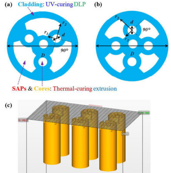
Fig. 2. Designed structures: (a) 3-core cross-section, (b) 4-core cross-section with 90^\circ bow-tie SAPs, both featuring an eccentric marking core. Here, D , r_1 , r_2 , and d represent the outer cladding diameter, radius of the SAPs, and core diameter, respectively; (c) openings at the starting end of the preforms.
