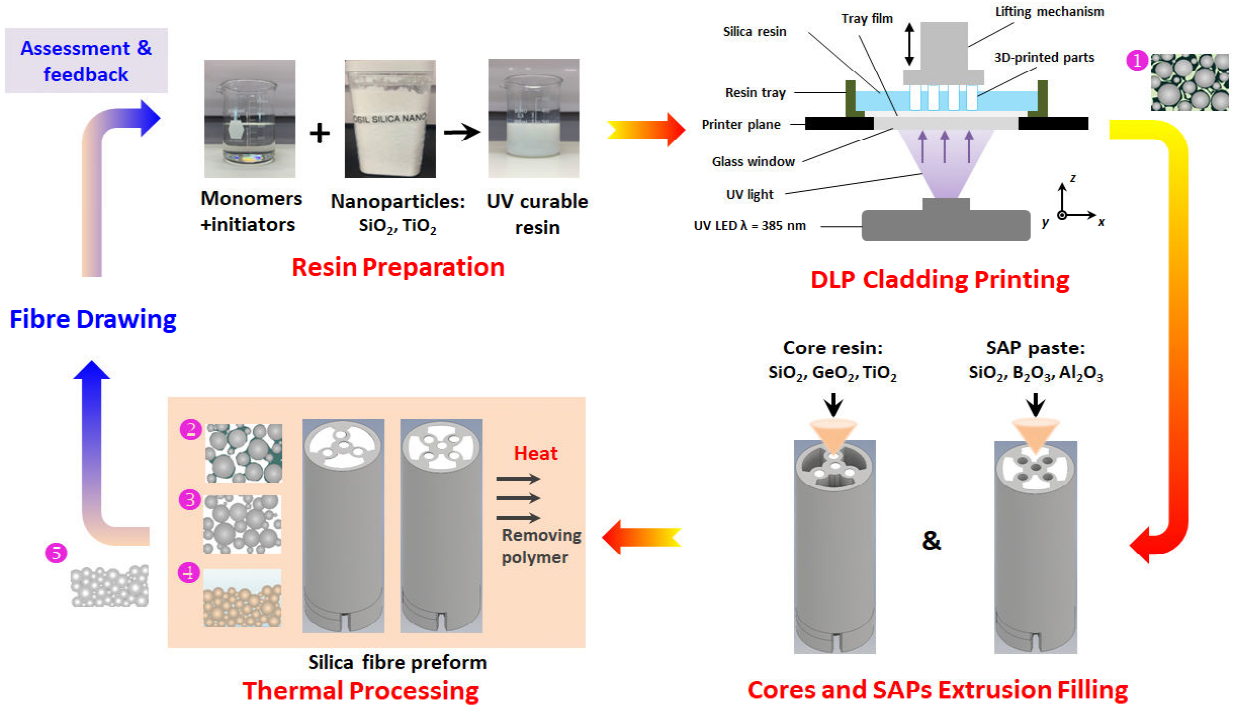
Fig. 3. Pathway of Hi-Bi MC SOF fabrication from dual-curing resins, the small pellets shown in Insets ①~⑤ represent nano composites associated with SOFs.
