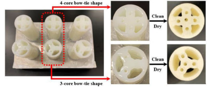
Fig. 5. Cladding parts with 3-core and 4-core bow-tie shape after DLP printing, cleaning and drying.
