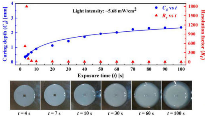
Fig. 4. Curing depth curve and distribution of photocuring resolution factors for the customized dual-curing resin, along with corresponding photos of the photocured parts at different exposure times.
