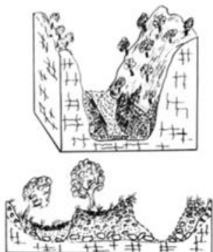
A. Confined, coarse textured
