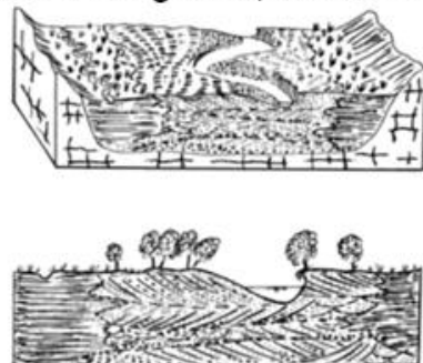
G. Lateral migration, backswamp
