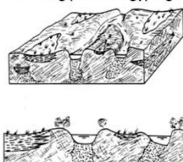
J. Anabranching (low energy) organic rich
