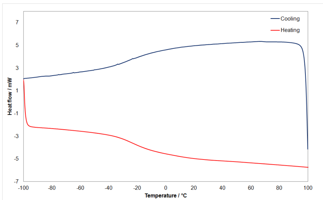
Fig. 11. Differential scanning calorimetry thermogram of \beta CPCD1 from -100\text{ }^{\circ}\text{C} to 100\text{ }^{\circ}\text{C} ( 10\text{ }^{\circ}\text{C min}^{-1} , third temperature cycle, aluminium crucible).
