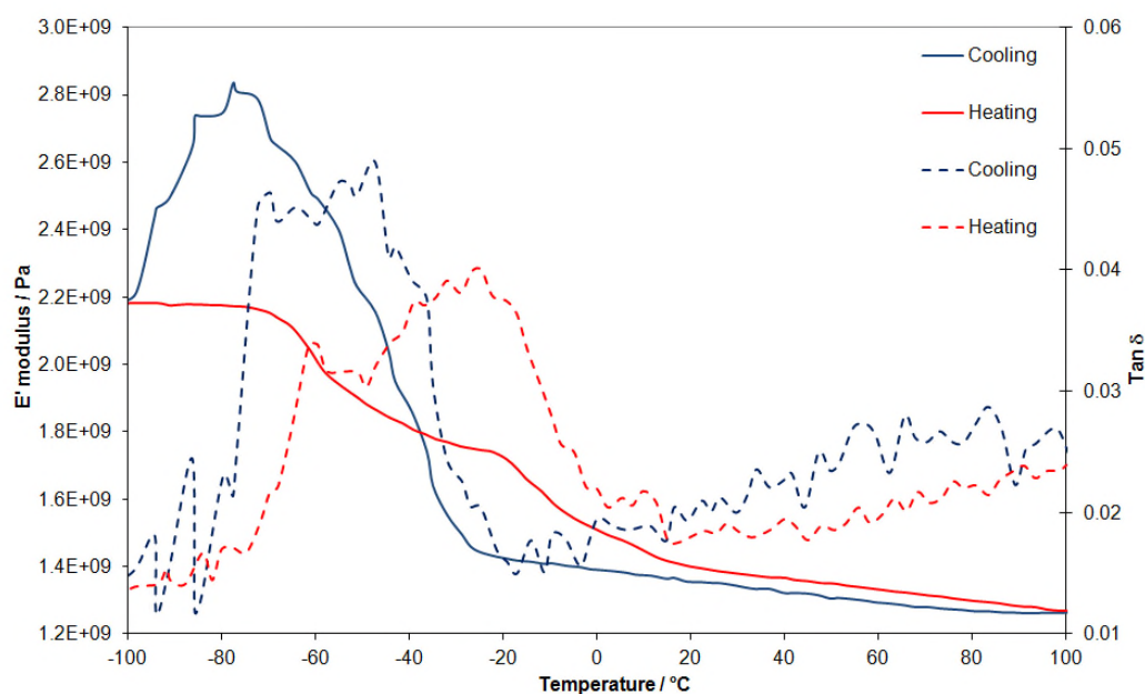
Fig. 6. Dynamic mechanical analysis showing the variation of the storage modulus ( E' ) (solid lines) and \tan \delta (dashed lines) of PEGDGE ( 10^\circ\text{C min}^{-1} , 1 Hz, third temperature cycle from -100^\circ\text{C} to 100^\circ\text{C} , aluminium pocket).
