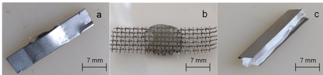
Fig. 3. Photographs of \beta CPCD samples supported by a) an aluminium pocket, b) a stainless-steel mesh, and c) an aluminium pocket wrapped in PTFE tape.
