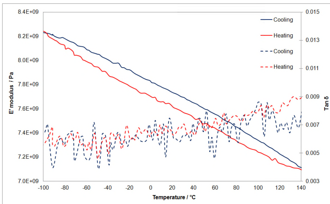
Fig. 4. Dynamic mechanical analysis showing the variation of the storage modulus ( E' ) (solid lines) and \tan \delta (dashed lines) of \beta CD ( 10\text{ }^{\circ}\text{C min}^{-1} , 1 Hz, third temperature cycle from -100\text{ }^{\circ}\text{C} to 140\text{ }^{\circ}\text{C} , aluminium pocket).
