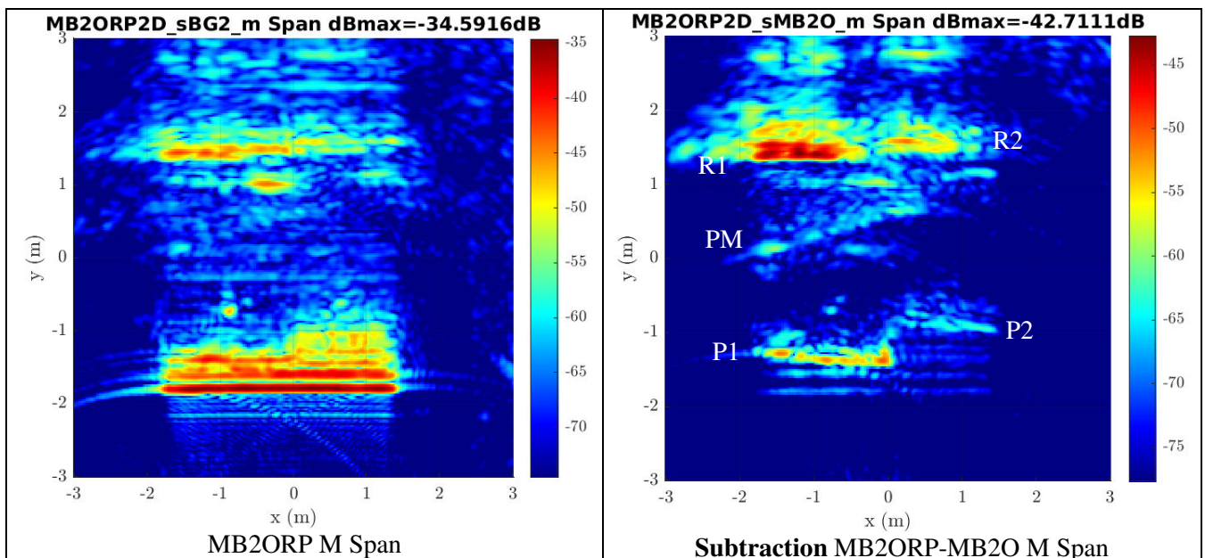
Figure 3-6. polarimetric Span monostatic images of MB2ORP (left) and subtraction MB2ORP-MB2O (right). The pipes (P1, P2) and the radiators (R1, R2) are marked on the subtraction image.
