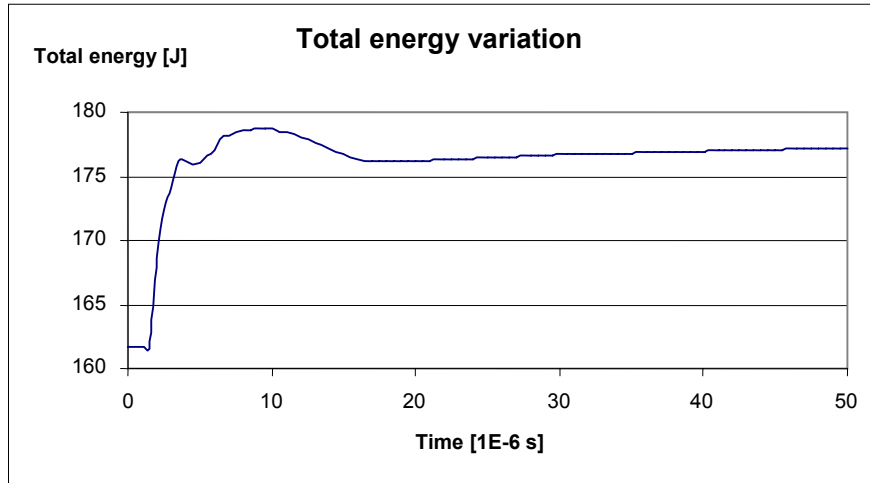
Figure 3: Total energy variation ( V_{imp}=817 m/s)
