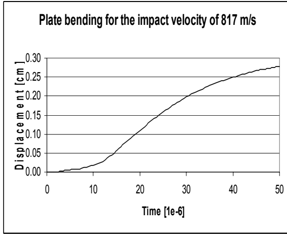
Figure 5: Negative Z displacement of the node marked in Figure 4
