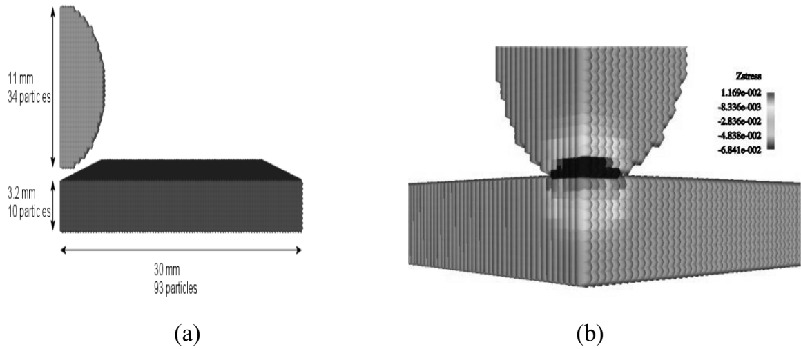
Figure 1: (a) SPH model for the MCM code (b) Z-stress state at time 0.6 μs. Unit: 10 2 GPa. ( V_{imp}=817 m/s)
