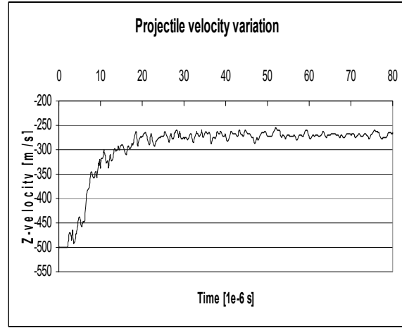
Figure 9: Projectile velocity vs. time
