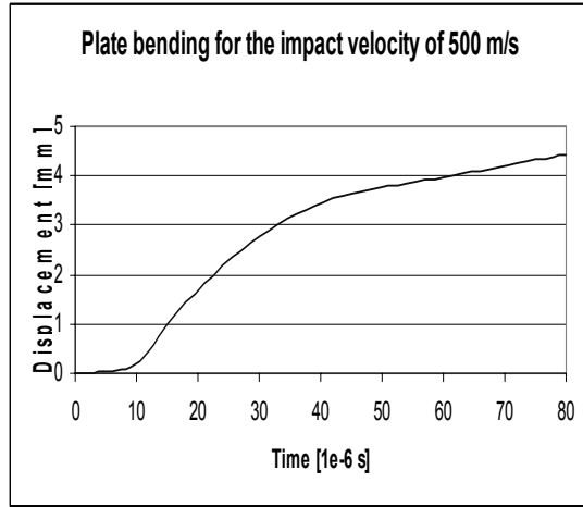
Figure 8: Displacement of the node marked “A” on Figure 6. ( V_{imp} = 500 m/s)
