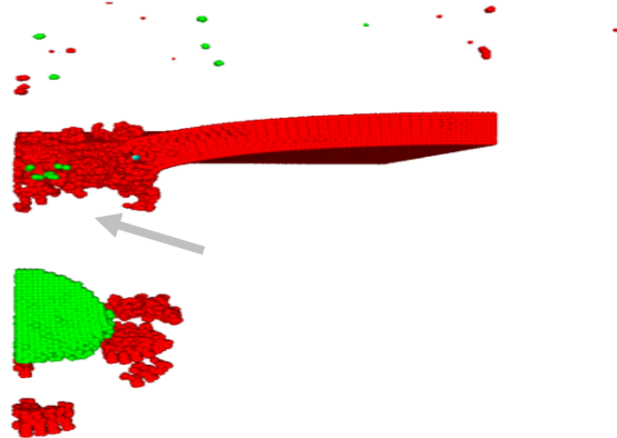
Figure 4: Projectile-target configuration at time 50 \mu s ( V_{imp}=817 m/s). The arrow points to the node whose displacement is plotted in Figure 5
