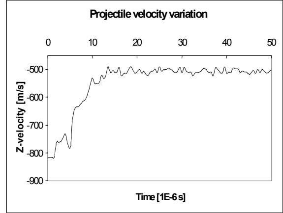
Figure 6: Projectile velocity vs. time ( V_{imp}=817 m/s)
