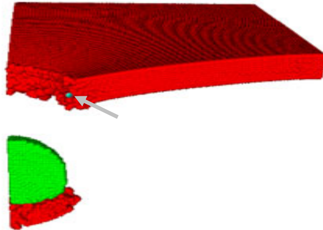
Figure 7: Configuration at time 80 \mu s ( V_{imp}=500 m/s). The arrow points to the node whose displacement is plotted in Figure 8.
