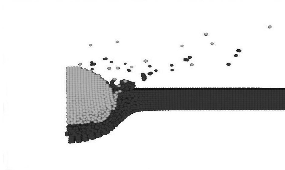
Figure 2: Projectile-target configuration at 15 μs.
