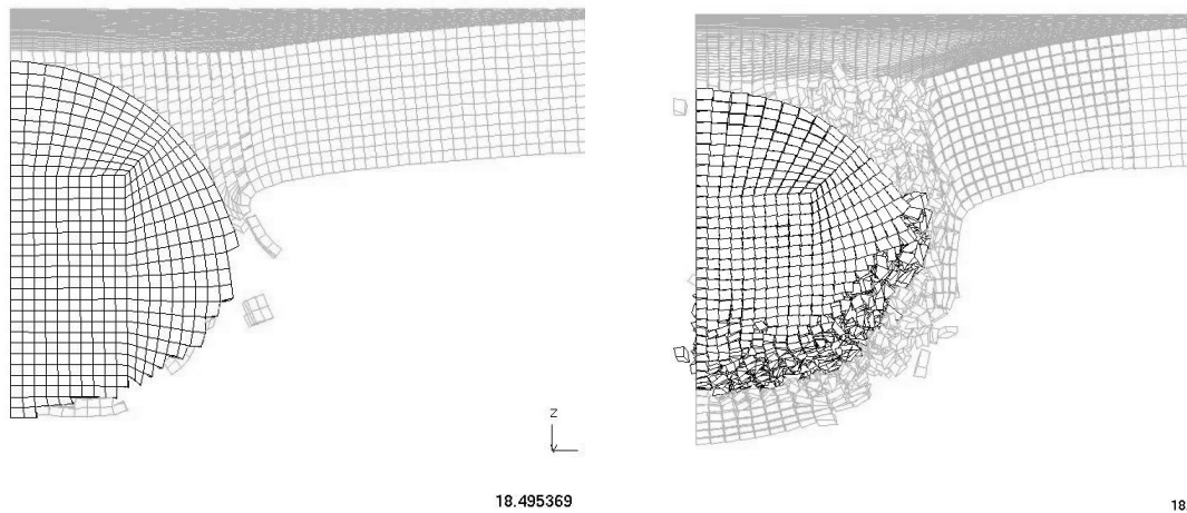
Figure 10: Comparison of the deformation predicted by element erosion method (LHS) and discrete element method (RHS) at time 18.5 \mu s. ( V_{imp} = 817 m/s)
