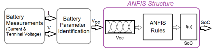
Fig. 10: Battery measurement, identification and SoC estimation
