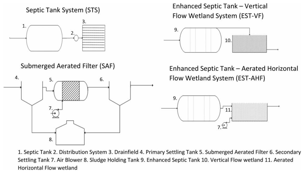
Figure 1 | Illustration of the analysed wastewater treatment flowsheets.
