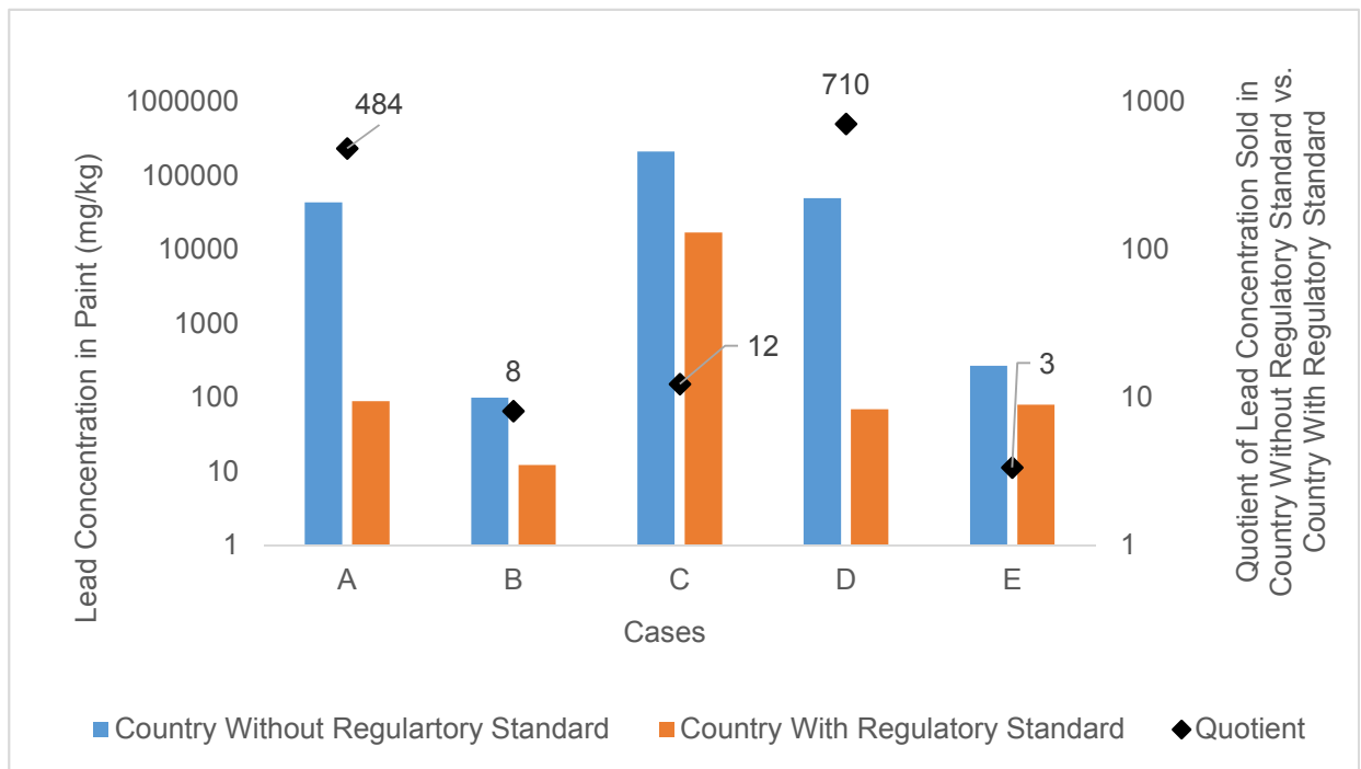
Figure 4 Lead levels in paints of the same brand and same colour being sold in developing countries with no regulatory standard vs. those sold in developing countries with voluntary regulatory standards (data source: (Betne et al. 2011))
