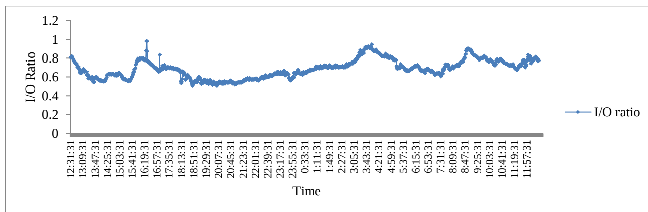
Fig.3. I/O ratio of PM 2.5 for Classroom III and Outdoor III
