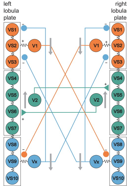
Figure S6: Putative synaptic coupling diagram of VS- and V-cells. Illustration of known (86) and hypothesized connections between the 10 VS-cells (VS1-VS10) and heterolateral V-cells (V1, V2, Vx) of the left and right lobula plate of the blowfly Calliphora . Colour coding corresponds to the proposed functional clusters shown in Fig. 2. Spherical and triangular symbols at the endpoints of connecting lines indicate inhibitory(-) and excitatory(+) outputs of the cells. Resistance symbols between cells refer to electrical synapses. Grey arrows indicate main sensitivity to vertical downward and upward motion of the LPTCs in the three clusters.
