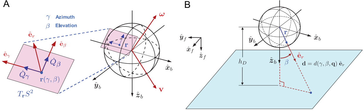
Figure S2: Geometry for spherical optic flow. (A) The azimuth \dot{Q}_\gamma and elevation \dot{Q}_\beta components of the optic flow vector are the projected relative velocities \omega and \mathbf{v} of visual contrasts or objects in the environment into the tangent space T_{\mathbf{r}}S^2 of the imaging surface, modeled here as a sphere approximating the nearly 4\pi visual field of the compound eyes. (B) The function d(\gamma, \beta, \mathbf{q}) is the distance from the imaging surface ( \mathbf{r} ) to the nearest point in the environment.
