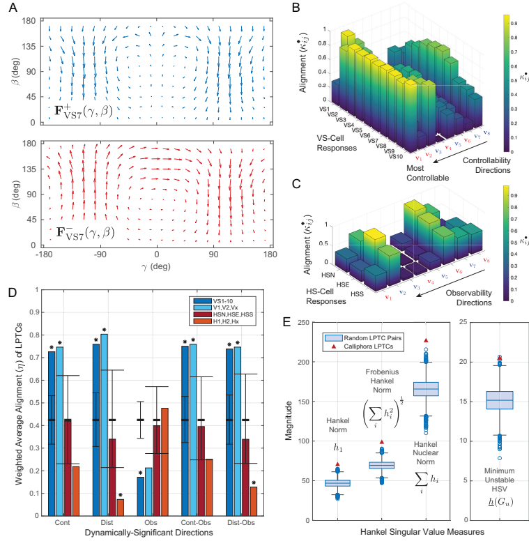
Figure 4: Functional principles of blowfly sensorimotor design. (A) Each LPTC pair carries separable information on symmetric versus asymmetric motion, which we illustrate by taking the sum (blue) or difference (red) of their response fields, shown here for VS7. (B,C) These response fields encode the cells' preferred directions of rotational and translational self-motion, which the mode-sensing hypothesis predicts will be aligned to dynamically-significant directions in the insect's state space. To test this, we quantified their alignment to the ordered symmetric (blue) or asymmetric (red) eigenvectors of the controllability and observability Gramians \{\mathbf{v}_1, \dots, \mathbf{v}_8\} , ranked by their dynamical significance (data in Tables S8,9). Collectively, the VS-cells strongly encode all of the most-controllable directions of symmetric/asymmetric motion, whereas the HS-cells strongly encode only the most-observable direction of symmetric motion. (D) Averaging over each LPTC sub-population, the V- and VS-cells strongly encode the directions that maximize controllability or disturbance-sensitivity both independently and jointly with observability; stars (*) denote statistical significance controlling the overall Type I error at \alpha = 0.05 . Note that no LPTC sub-population is aligned to the most-observable directions of motion, as would be conventional in engineering design. (E) To assess overall system performance, we computed four measures (the Hankel norm, the Frobenius-Hankel norm, the Hankel Nuclear norm, and the minimum unstable) of the Hankel singular values \{h_1, \dots, h_8\} characterizing signal energy flow through the system for all 19 LPTC pairs (red points) and compared these to the Hankel singular values of 10,000 randomly-generated sets of preferred directions (blue box plot; whiskers extend \pm 2.7 S.D.). The blowfly's Hankel singular values are far higher than expected by chance, demonstrating that the LPTCs' tuning maximizes signal energy flow through the system. The first Hankel singular value provides an upper bound on signal energy flow from input to output, and is higher for the
