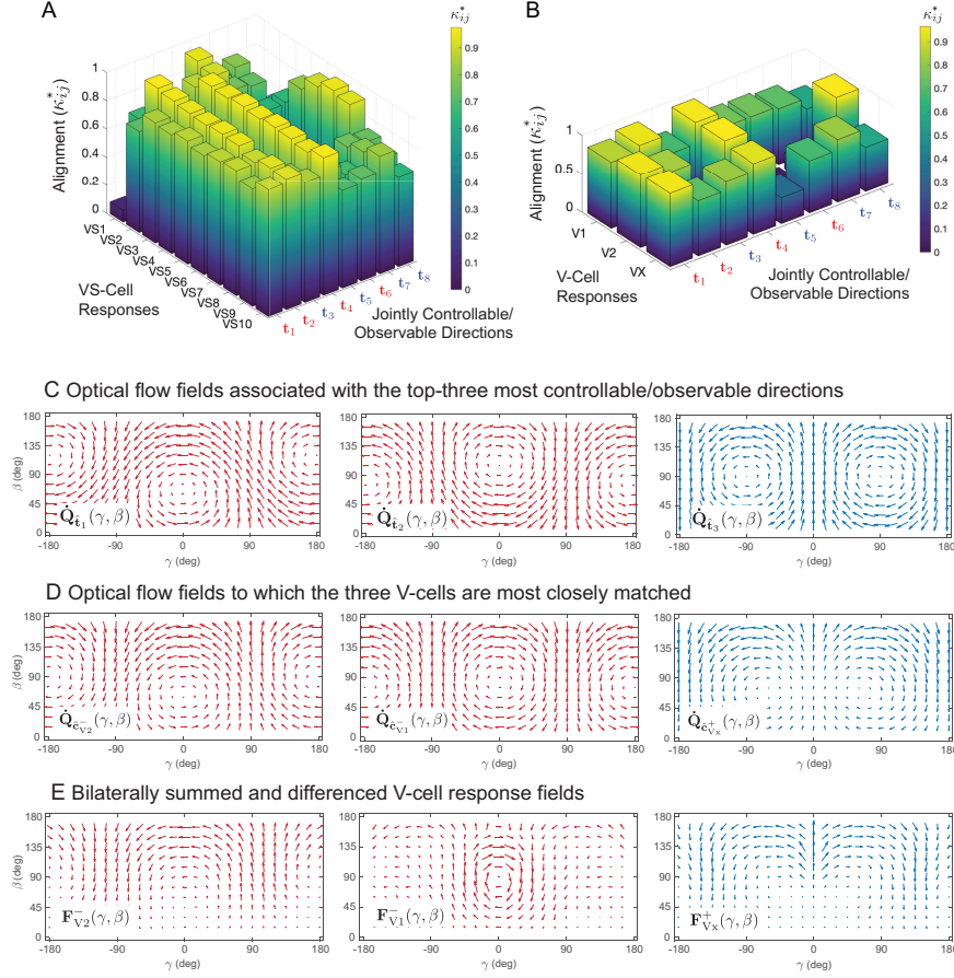
Figure 5: Tuning of the vertical system LPTCs to the fly's jointly controllable/observable directions of self-motion. (A,B) Signal energy flow is maximized when a system's sensors are matched to its most-controllable/observable directions of self-motion. To demonstrate the closeness of this tuning in the blowfly, we first quantified the alignment of the preferred directions of the LPTCs to the ordered symmetric (blue) or asymmetric (red) column vectors \{t_1, \dots, t_8\} of the inverse balancing transformation matrix. These vectors span the entire controllable/observable subspace of the insect, and the bilaterally summed and differenced response fields of the VS- and V-cell pairs are shown to be strongly aligned with them all (data in Tables S10,11). (C-E) To demonstrate this visually, we also computed the re-projected optic flow fields corresponding to: (C) the top three most controllable/observable directions of symmetric (blue) or asymmetric (red) self-motion; and (D) the preferred directions of symmetric (blue) or asymmetric (red) self-motion for the three V-cell pairs. Note the closeness of the match. (E) The summed and differenced response fields of the V-cell pairs also resemble the re-projected optic flow fields corresponding to the joint most-controllable/observable directions of motion, but do so less closely owing to spatial variation in the cells' local motion sensitivity, which is expected to embed a nearness distribution corresponding to a natural environment (16).
