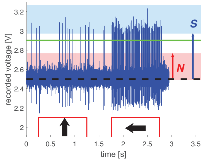
Figure S1: Signal-to-Noise ratio in extracellular recordings from spiking LPTCs. The voltage during an H1-cell recording is plotted over time. Red rectangles (bottom) indicate stimulus time intervals of upward and back-to-front movement of a local visual grating centred at +15^\circ azimuth and elevation. The setpoint of the extracellular amplifier is at 2.5 volt (dashed black line). S and N indicate the signal- and noise- bands of the recorded voltage, respectively. For ratios of S/N > 2 , a simple threshold criterion can be applied to reliably detect the spikes generated by the H1-cell ( S band) without contamination from background signals in the noise band ( N ). The threshold voltage used during the recording shown was set to 2.9 Volt (solid green line). Only signals greater this voltage amplitude were identified as the H1-cell spikes.
