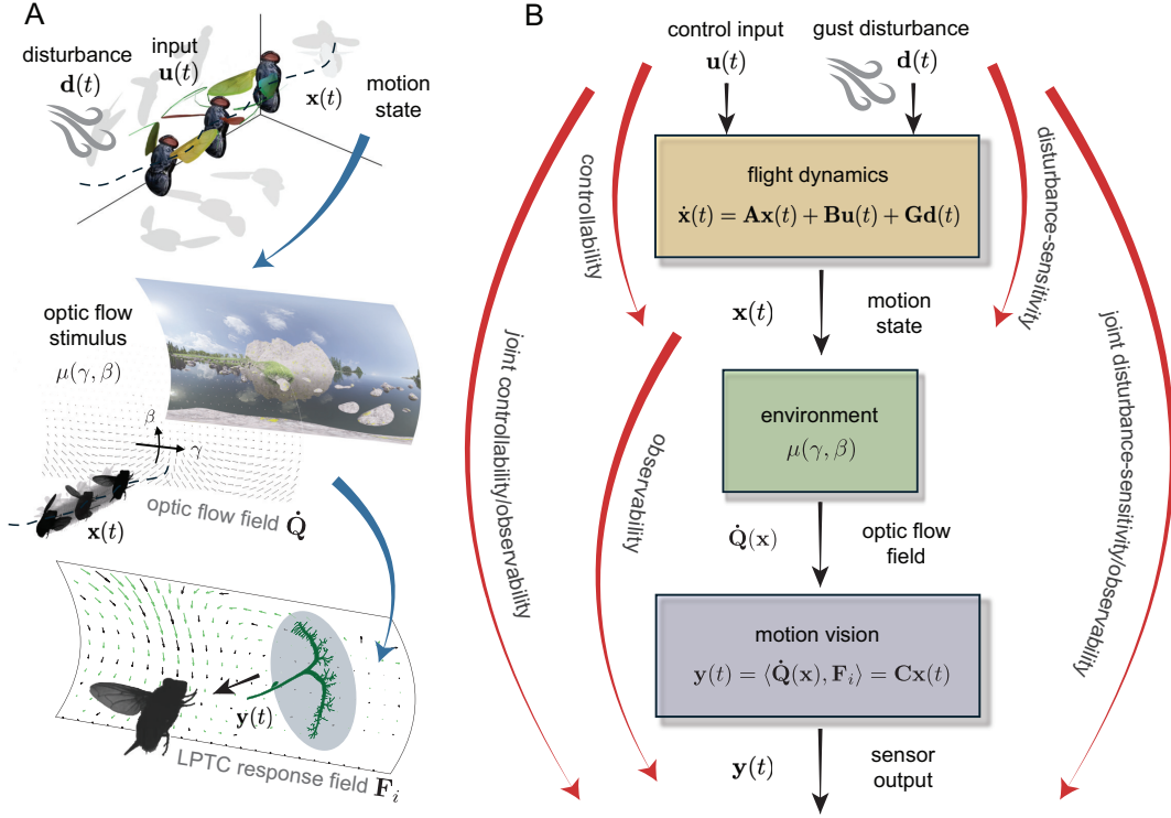
Figure 1: Signal energy transfer in insect flight. The mechanistic relationships illustrated in (A) (blue arrows) are summarised by the signal energy flows shown in (B) (red arrows). We characterise these mechanistic relationships by developing a state-space model of insect flight (Eqs. 1-2), and characterise the associated signal energy flows using the matrix structures (Gramians) derived from this model (Eqs. 3–4). Blue arrows: Control inputs u(t) and gust disturbances d(t) produce changes in the insect’s motion state x(t) described by the differential equations characterising its flight dynamics. This self-motion generates sensory stimuli including an optic flow field through interaction with the local nearness \mu(\gamma, \beta) of the environment. The output layer of the blowfly motion vision system comprises a set of lobula plate tangential cells (LPTCs), each of which is matched to detect an optic flow field associated with a specific self-motion, yielding a sensor output y(t) related to the motion state x(t) of the fly. Red arrows: Signal energy from control inputs and gust disturbances is stored in the system state, so the system’s controllability and disturbance-sensitivity are maximized by maximizing signal energy storage. Stored signal energy is released through the evolution of the system state and retrieved at the sensor outputs, so the system’s observability is maximized by maximizing signal energy retrieval. A system that balances signal-energy storage/retrieval jointly maximizes observability and controllability or disturbance-sensitivity, and thereby maximizes the flow of signal energy from control inputs or gust disturbances to sensor outputs via the system state.
