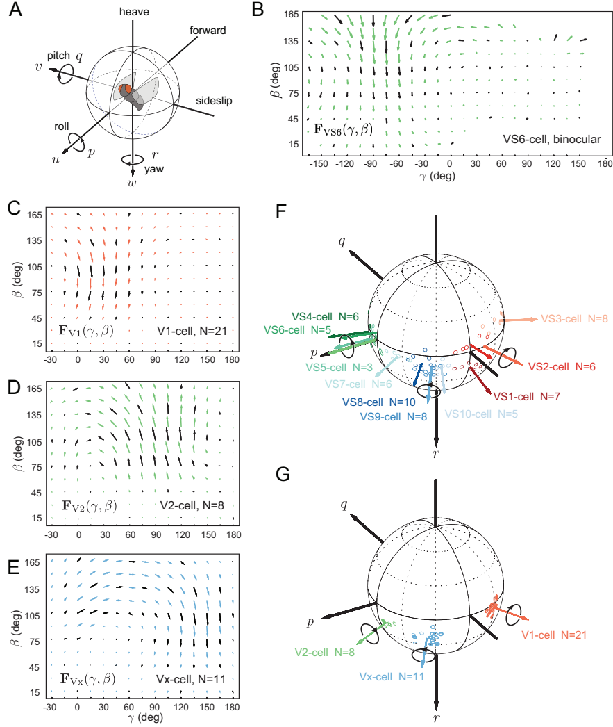
Figure 2: The fly motion vision system. (A) A flying insect has six degrees of freedom in rotation \{p, q, r\} and translation \{u, v, w\} . Its compound eyes sense self-motion using a deep network comprising an array of repeated elementary motion detectors whose outputs are pooled by the lobula plate tangential cells (LPTCs). LPTCs build an output layer of 13 pairs of VS- and HS-cells connected by a hidden layer of at least 6 pairs of V- and H-cells coupling the left and right optic lobes. (B) Binocular response field of the left VS6-cell showing the neurons local preferred directions and motion sensitivities as a function of azimuth ( \gamma ) and elevation ( \beta ) in retinal coordinates. This closely resembles the optic flow associated with left-handed roll motion (27), and as the LPTCs only arborize ipsilaterally, the weak contralateral response visible here must be due to coupling by the heterolateral V-cells. (C,D,E) Newly-measured response fields of the right V-cells, where N denotes the number of individuals from which the recordings were pooled. (F,G) Preferred rotation axes of the left VS- (15, 25) and V-cells (new data); cells of the right optic lobe have responses that are mirror-symmetric to those of the left optic lobe. Long colours arrows in F and G give the average preferred rotation axis of the functional groups VS1-3; VS4-7 and VS8-10 as well as the spiking V1, V2, and Vx cells, respectively. Black circular arrows indicate preferences for clockwise or counterclockwise rotations.
