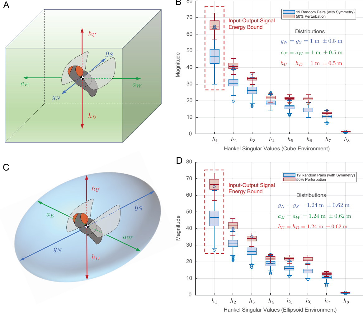
Figure S4: Robustness of Hankel singular values to environment perturbations. The dimensions (g_N, g_S, a_E, a_W, h_u, h_d) of two different nominal environment configurations with equal volume (cube, ellipsoid) are randomly selected from a uniform distribution (100 different configurations each) up to 50% and used to generate the system's Hankel singular values. These distributions are compared to 1000 sets of randomly selected 19 left-right symmetric pairs from a uniform distribution on \mathbb{R}^8 . (A) Geometry of the cube environment. (B) Comparison of Hankel singular values for 100 randomly selected cube environment configurations. (C) Geometry of the ellipsoid environment. (D) Comparison of Hankel singular values for 100 randomly selected ellipsoid environment configurations.
