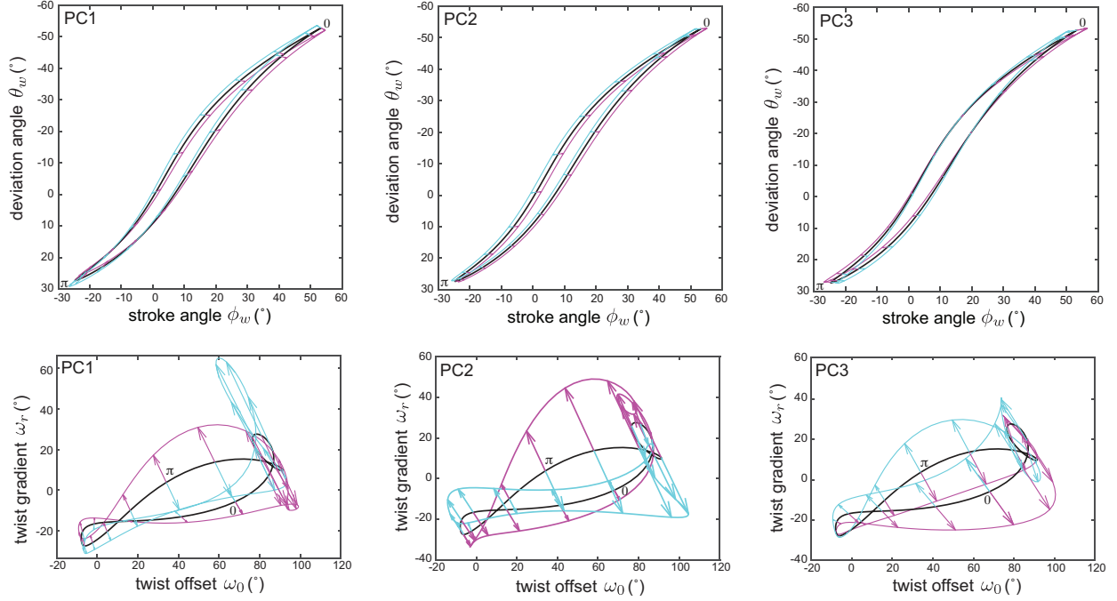
Figure S7: Principal components of wing kinematic perturbations. Phase-plane plots showing the variation in the time-periodic wing tip kinematics described by each of the first three principal components (PC1–PC3). Black lines display the mean wing kinematics over all the wingbeats that we measured; cyan and magenta lines display the effect of a \pm 1 SD perturbation in each PC; arrows connect points of equivalent phase. The point of dorsal stroke reversal is defined as phase \varphi = 0 ; the point of ventral stroke reversal corresponds approximately to phase \varphi = \pi . Note that the primary effect of perturbing the wing kinematics in the directions of PC1 and PC3 is to tilt the stroke plane with respect to the body axes, whereas PC2 describes a wholesale fore-aft displacement of the stroke plane. These changes in the wing tip kinematics are coupled with the changes in wing twist distribution.
