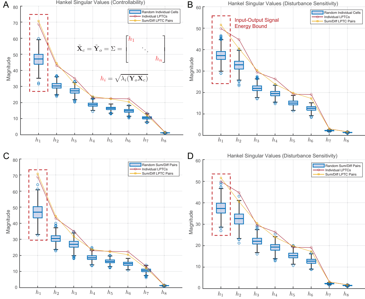
Figure S5: Hankel singular value dependence on LPTC configuration. Two different configurations (individual cells or bilaterally summed and differenced pairs) of the output vectors \mathbf{y}' and \mathbf{y} respectively are used to generate Hankel singular values for the controllability and disturbance sensitivity cases. These results are compared to two configurations (individual cells or bilaterally summed and differenced pairs) of 1000 randomly generated sets from a uniform distribution on \mathbb{R}^8 . The maximum Hankel singular value h_1 represents a bound on signal energy transfer from input to output. (A-B) Comparison of Hankel singular values based on the controllability Gramian X_c and the disturbance sensitivity Gramian X_d with randomly generated sets of 38 individual cells (19 symmetric pairs). (C-D) Comparison of Hankel singular values based on the controllability Gramian X_c and the disturbance sensitivity Gramian X_d with randomly generated sets of bilaterally summed and differenced pairs.
