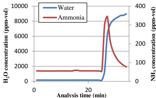
Figure 10 - Deconditioning of the instrument when \text{H}_2\text{O} is introduced into the instrument
