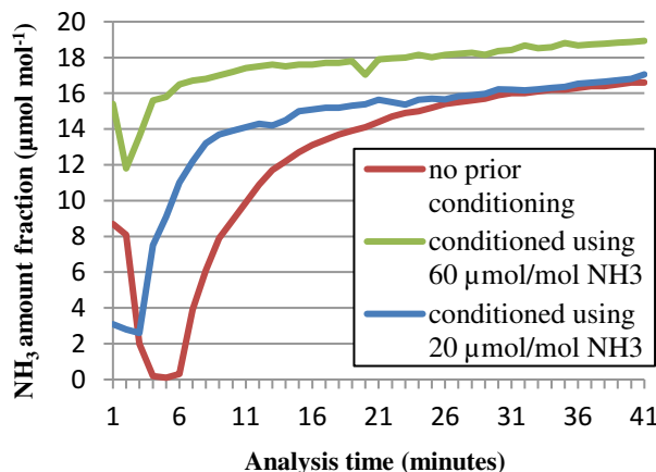
Figure 8 - Effect of conditioning the instrument prior to the analysis of biomethane for the determination of \text{NH}_3 concentration
