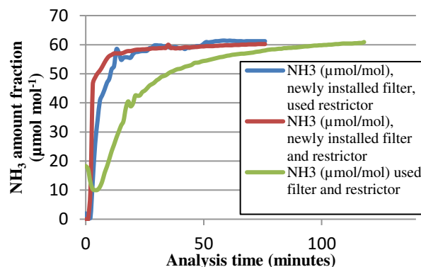
Figure 9 - Effect of filter condition when analysing biomethane for the determination of \text{NH}_3 concentration
