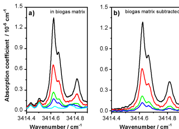
45 Figure 7 - Panel a) Recorded spectra of \text{NH}_3 in Biogas 40 (8.5 46 \mu\text{mol mol}^{-1} \text{NH}_3 , black), 3 dilutions with Biogas 40 (4.2 \mu\text{mol} 47 \text{mol}^{-1} , red), (1.4 \mu\text{mol mol}^{-1} , green), (0.7 \mu\text{mol mol}^{-1} , blue) and 48 pure Biogas 40 (teal). Panel b) Residual spectra following sub- 49 traction of the pure Biogas 40 spectrum.
