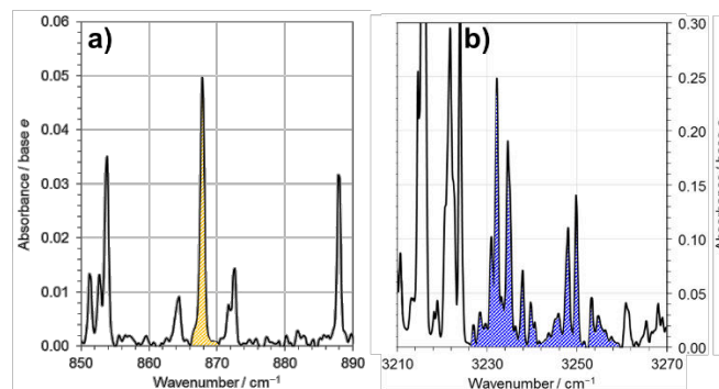
Figure 1 – FTIR spectra of trace ammonia in Biogas 20 at 0.5 cm -1 resolution, highlighting the integrated absorbance areas of a) NH 3 and b) CH 4 .
