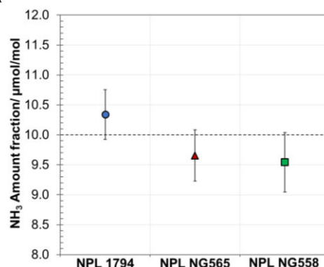
75 Figure 3 – Certified \text{NH}_3 amount fraction in the three 10 \mu\text{mol mol}^{-1} \text{NH}_3 in biogas mixtures used in the stability study. The error bars represent an expanded uncertainty with coverage factor k = 2 . The dashed line indicates the gravimetric \text{NH}_3 amount fraction in the three mixtures.
