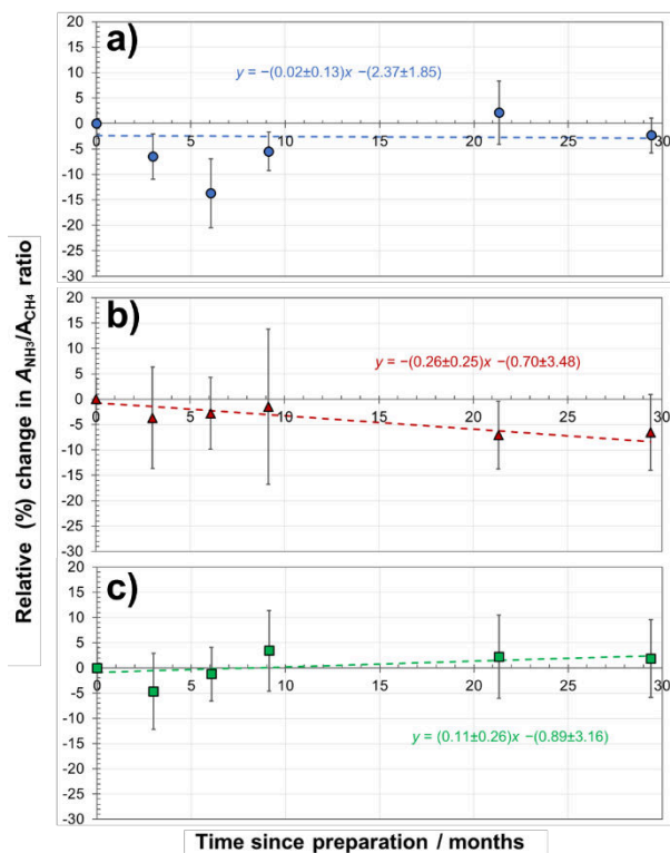
32 33 Figure 2 – Stability of 10 \mu\text{mol mol}^{-1} \text{NH}_3 mixtures in: a) \text{CH}_4 34 (NPL1794), b) Biogas 20 (NPL NG565) and c) Biogas 40 (NPL
