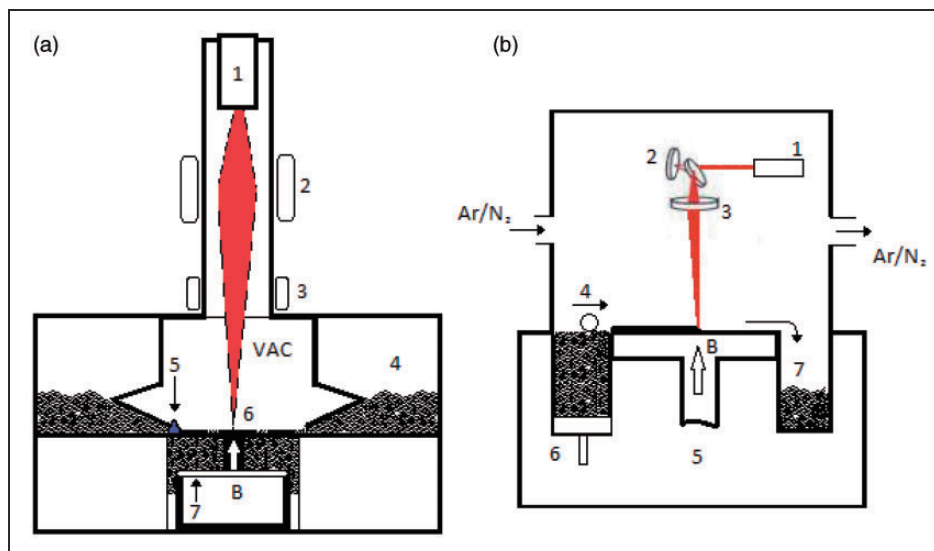
Figure 2. EBM (a) and SLM (b) systems schematics.
