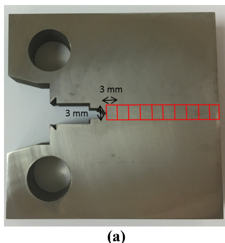
Fig. 9. (a) Extraction pattern of the strain free samples for d_o measurements (b) Strain free cube samples numbered from 1 to 10.
