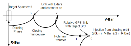
Fig. 24. R-bar proximity orientations and docking.
