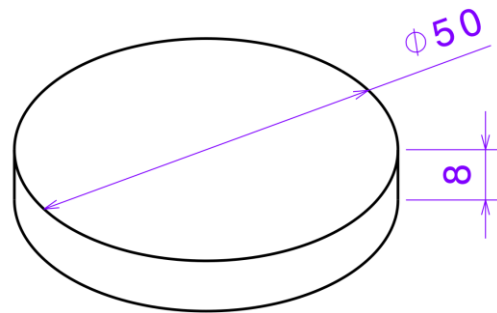
Figure 1. Specimen dimensions.
