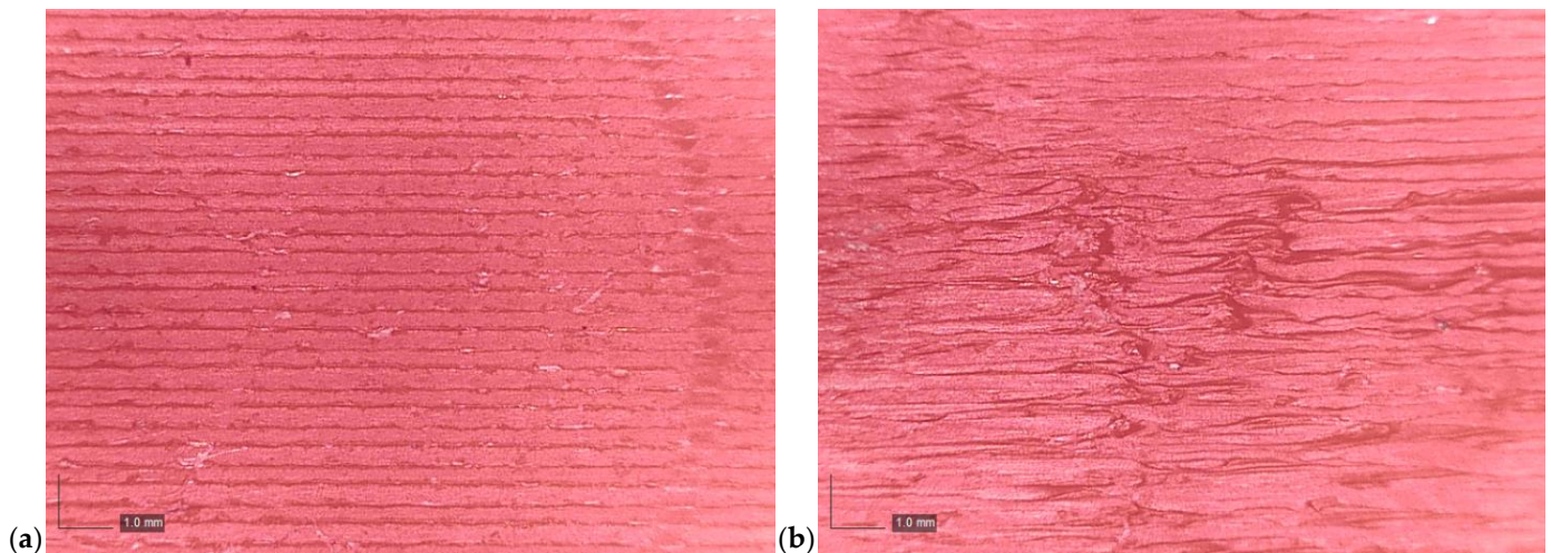
Figure 5. Microscope images showing surface morphology at different layer heights: (a) 0.20 mm and (b) 0.35 mm.
