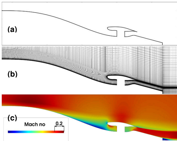
Figure 6: Design selected for the grid sensitivity analysis: (a) geometry of the model, (b) Mesh B, 4.43 \times 10^5 elements, and (c) Mach number contour
