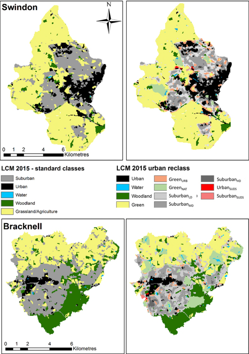
Figure 3: Comparison of land cover classes using standard and refined urban reclassification for both Swindon and Bracknell town (2015)
