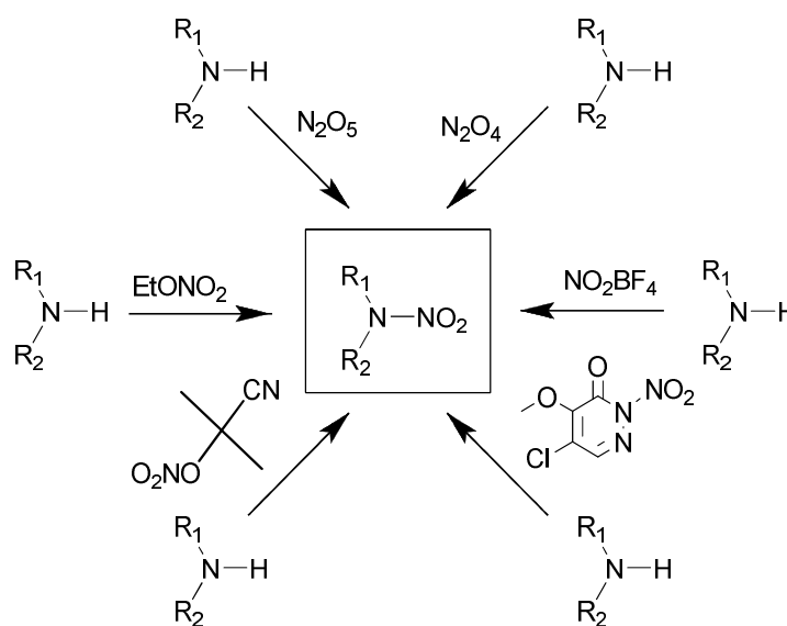
Figure 6: Nitrating agents
