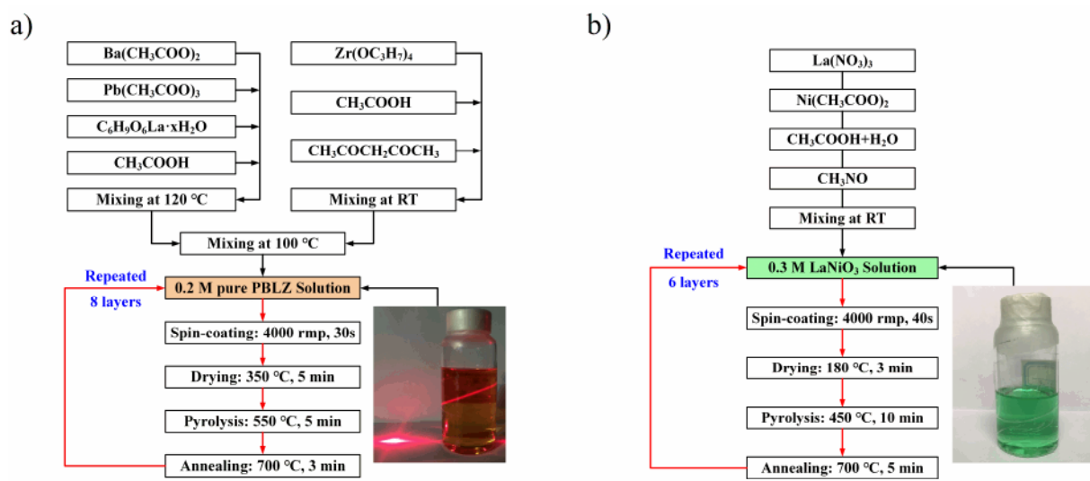
Fig.S1. Flow charts of the preparation of (a) \text{Pb}_{0.78}\text{Ba}_{0.2}\text{La}_{0.02}\text{ZrO}_3 (PBLZ) thin films and (b) \text{LaNiO}_3 bottom electrode.
