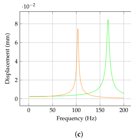
Figure 12. Steady-State Dynamics Analysis Plots. (a) Frequency Response to 2.2G in +X; (b) Frequency Response to 2.2G in +Y; (c) Frequency Response to 15G in +Z.
