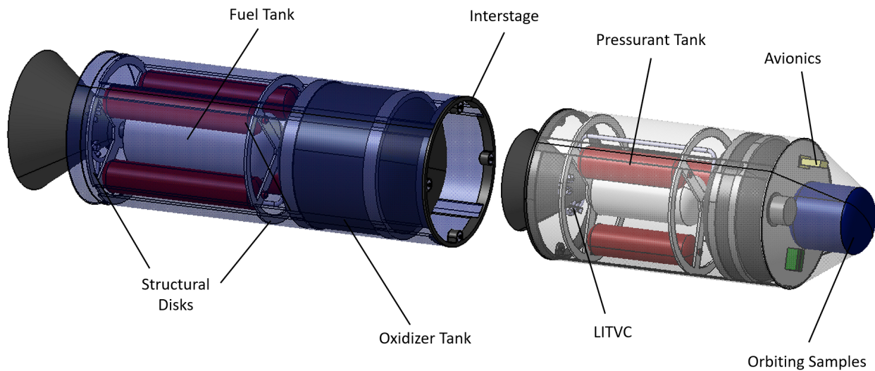
Figure 3. Hybrid MAV Configuration.
