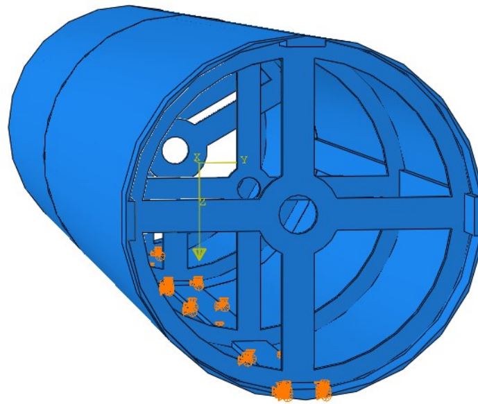
Figure 6. Boundary Conditions FEA. The orange arrows represents the boundary conditions, the yellow arrows represent the reference frame, and the blue the part analysed, which is the primary structure.
