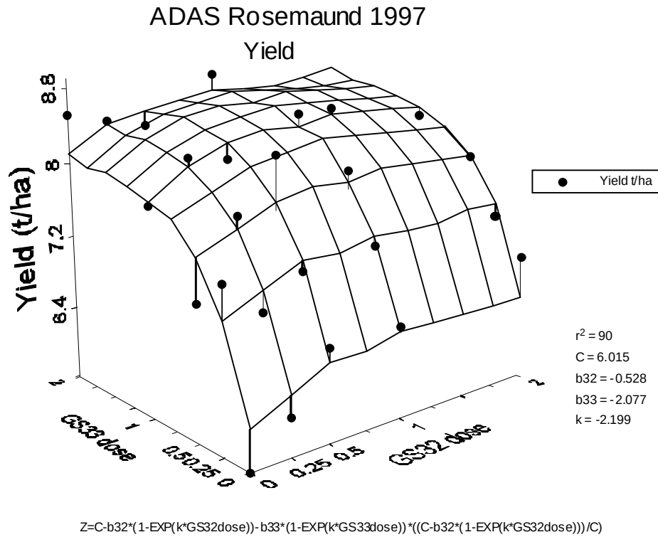
1 Fig. 5. Dose-response surface for two applications of tebuconazole fitted to data from an 2 experiment at Rosemaund in the 1996/1997 season. The first application was carried out 3 as leaf III emerged and the second as leaf II emerged. The yield data points that the 4 surface was fitted to (Eqn 17) are indicated by the solid dot (●). The dose is L ha -1 of 5 commercial product.
