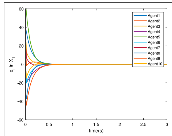
Figure 6. Error in X_1 calculated using non-linear dynamic inversion (Case 1).
