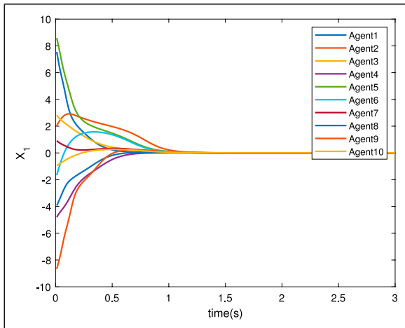
Figure 2. Consensus of state X_1 (Case 1).
