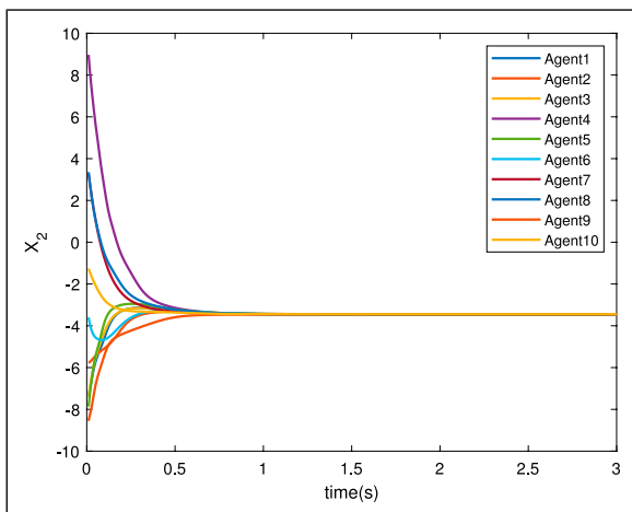
Figure 3. Consensus of state X_2 (Case 1).
