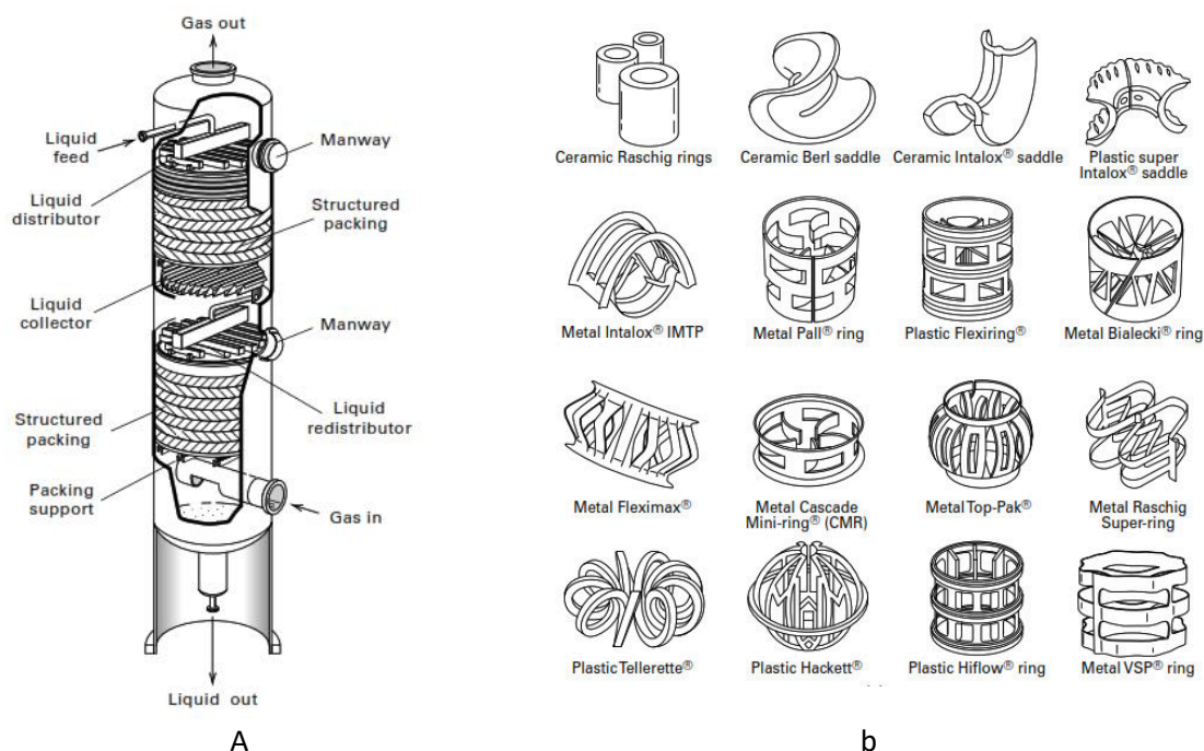
Figure 1. Typical wet type gas scrubber (a) design and (b) typical materials and shape designs used in construction of a packed column (Seader et al., 2011).
