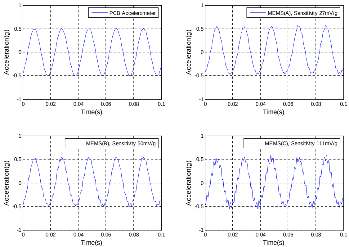
Figure 5 Measured acceleration responses by the MEMS accelerometers and the reference (PCB) accelerometer at 53Hz for the excitation level 0.5g
