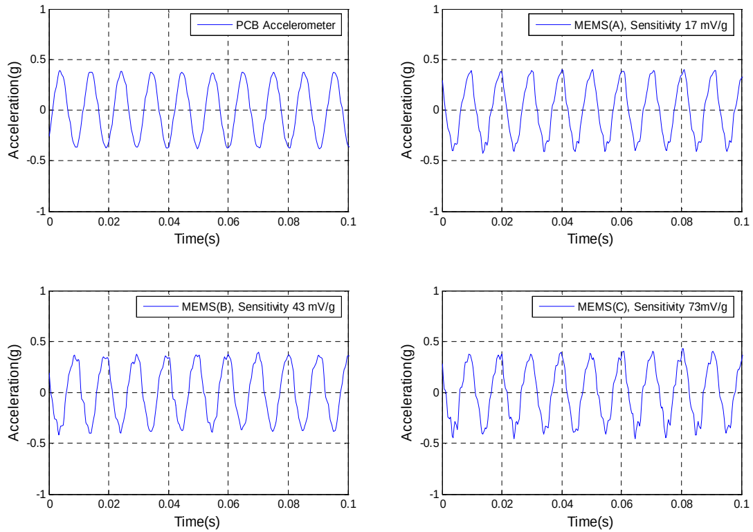
Figure 9 Measured acceleration responses by the MEMS accelerometers and the reference (PCB) accelerometer at 95Hz for the excitation level 0.35g
