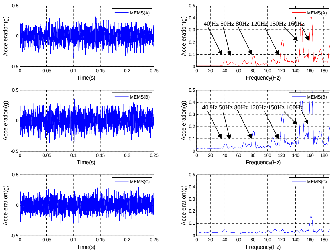
Figure 18 CNC machine vibration measured by the MEMS accelerometers at speed of 2400 rpm
