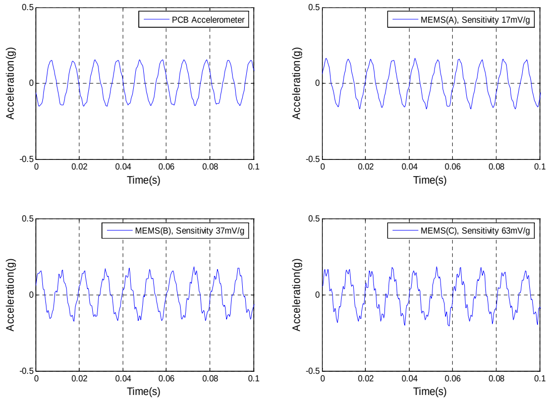
Figure 7 Measured acceleration responses by the MEMS accelerometers and the reference (PCB) accelerometer at 95Hz for the excitation level 0.15g
