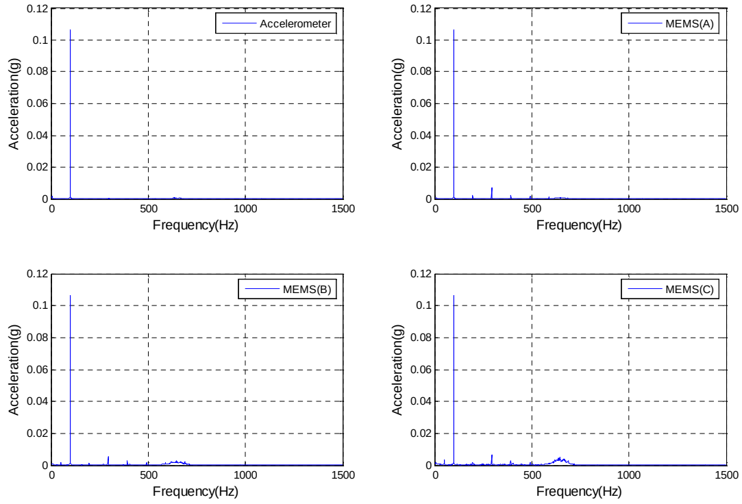
Figure 8 Frequency domain of the measured acceleration responses by the MEMS accelerometers and the reference (PCB) accelerometer at 95Hz for the excitation level 0.15g
