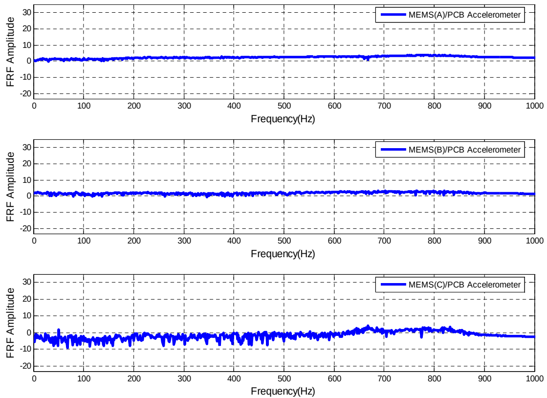
Figure 15 Frequency response function for the MEMS accelerometers
