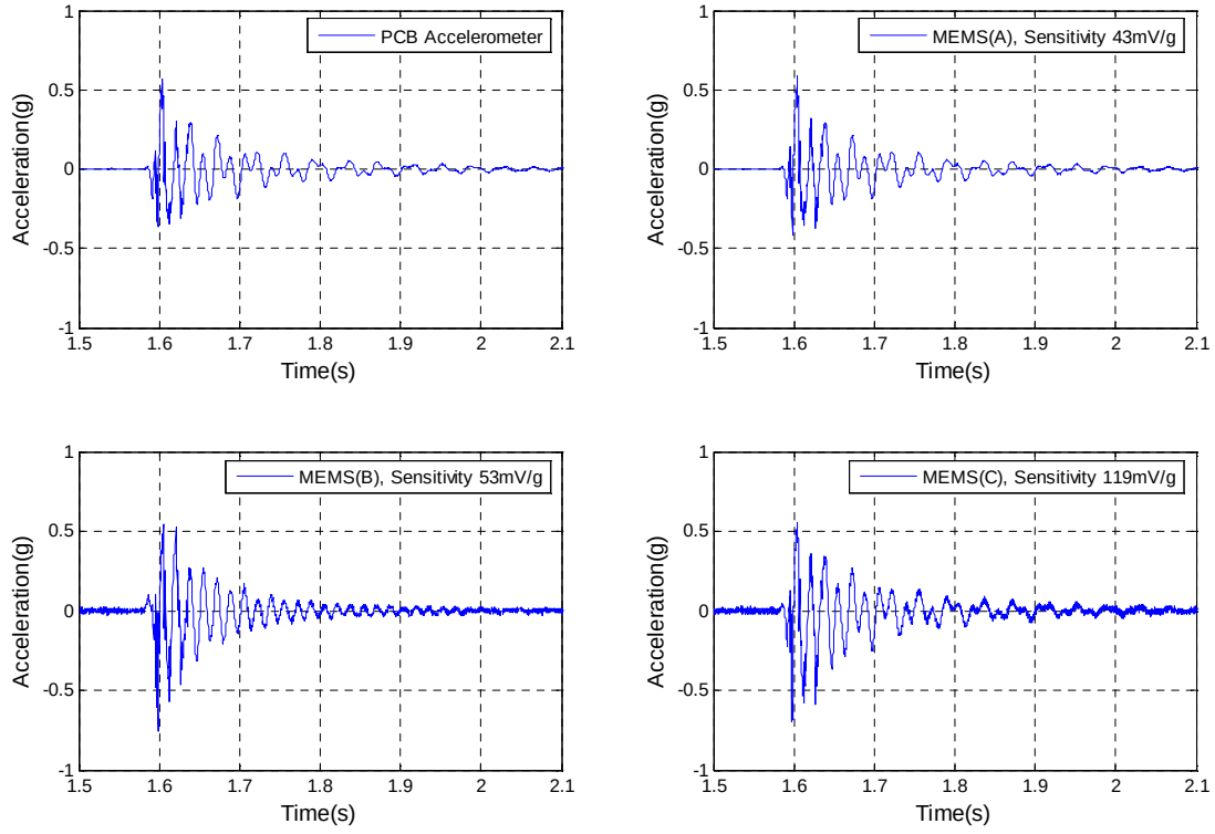
Figure 11 A comparisons of measured responses by the MEMS accelerometers and the reference (PCB) accelerometer using a soft tip hammer
