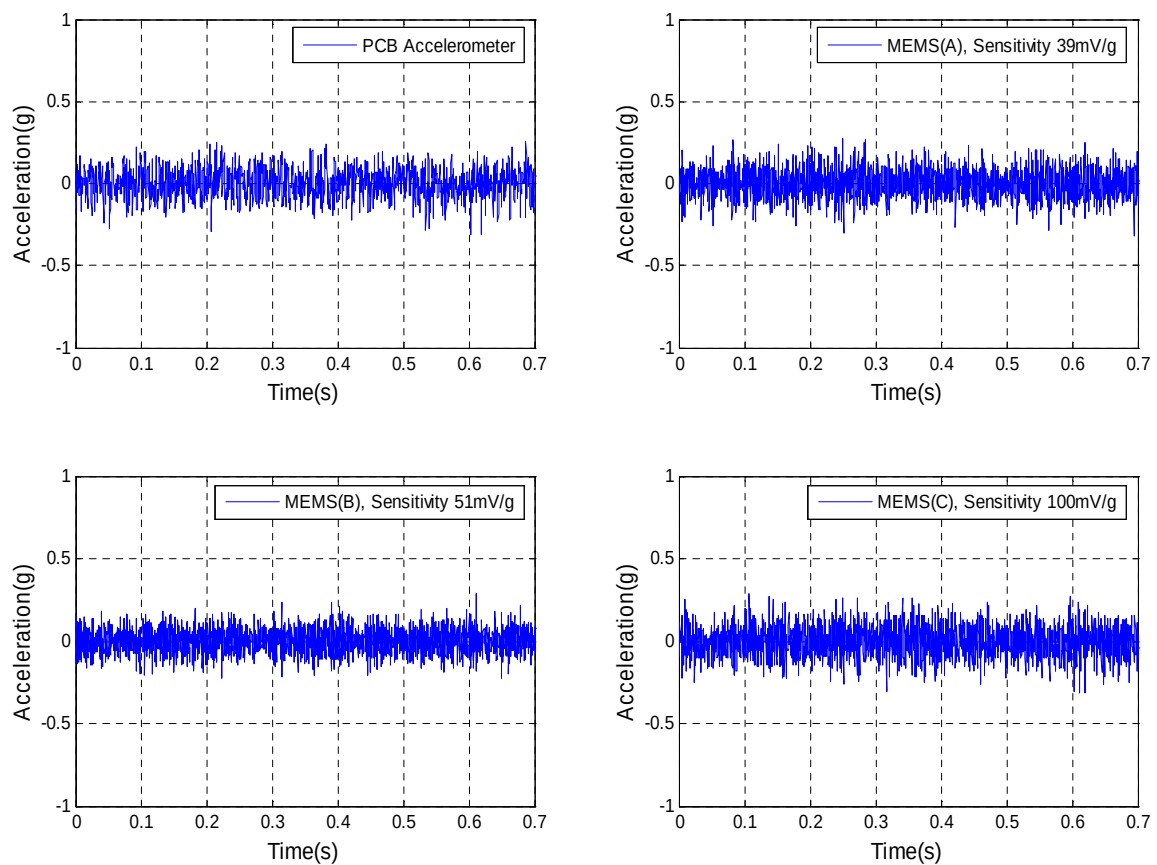
Figure 13 Time domain of accelerometers responses when the shaker is excited by a random noise
