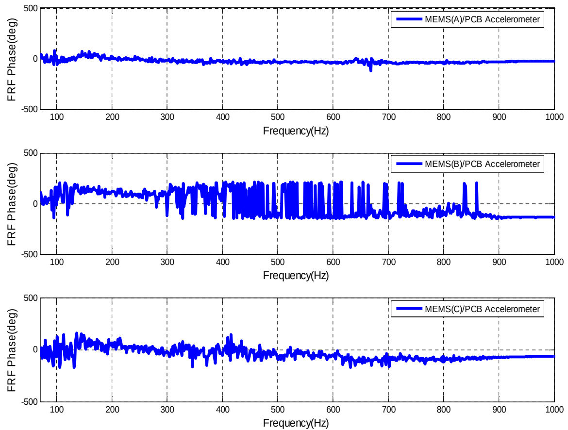
Figure 16 Phase of the frequency response function for the MEMS accelerometers
