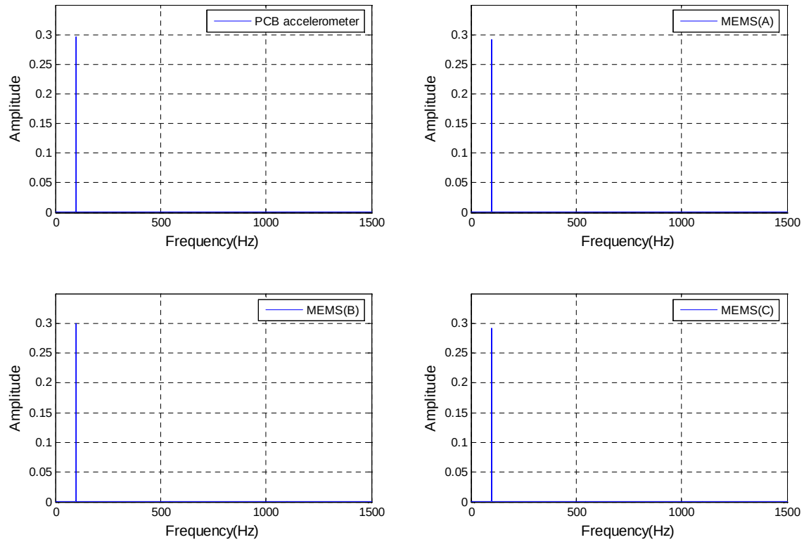
Figure 10 Frequency domain of the measured acceleration responses by the MEMS accelerometers and the reference (PCB) accelerometer at 95Hz for the excitation level 0.35g
