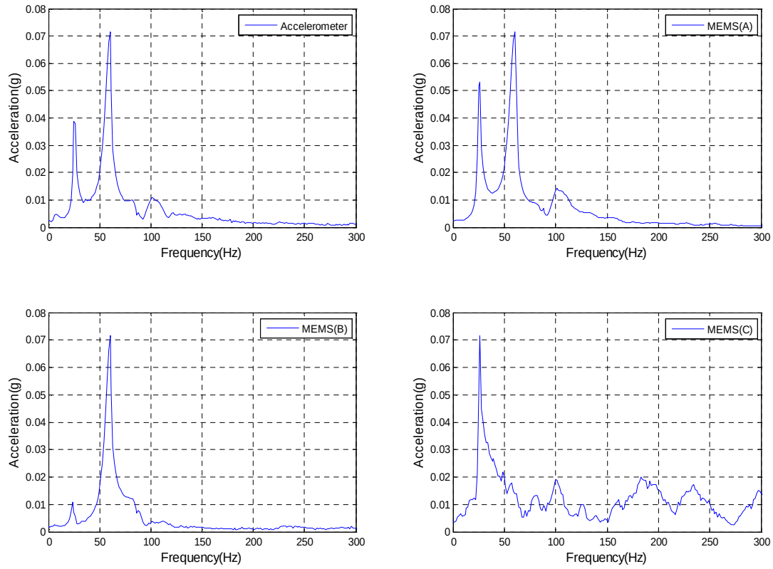
Figure 12 Frequency domain of the measured responses by the MEMS accelerometers and the reference (PCB) accelerometer using a soft tip hammer
