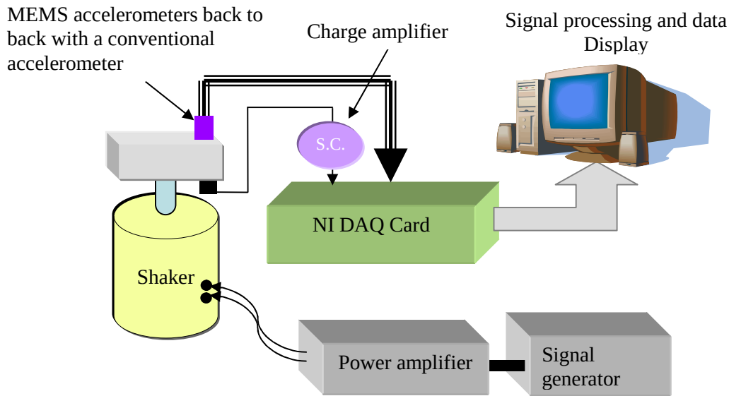
Figure 2 Test setup
