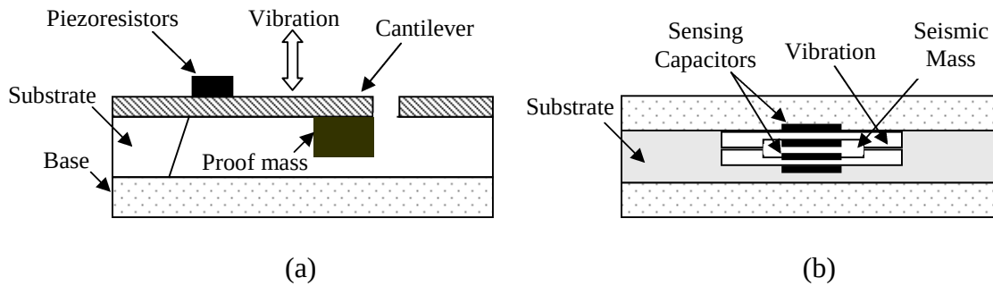
Figure 1 A typical MEMS accelerometer construction; (a) Piezoresistive using cantilever design, (b) capacitive based on membrane design [1]
