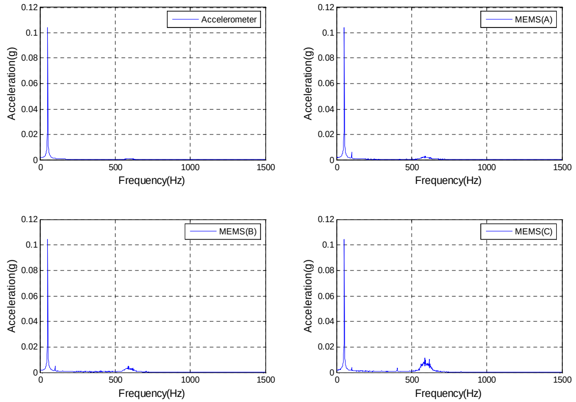
Figure 4 Frequency domains of the measured acceleration responses by the MEMS accelerometers and the reference (PCB) accelerometer at 53Hz for the excitation level 0.15g
