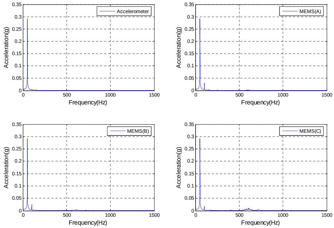
Figure 6 Frequency domains of the measured acceleration responses by the MEMS accelerometers and the reference (PCB) accelerometer at 53Hz for the excitation level 0.5g
