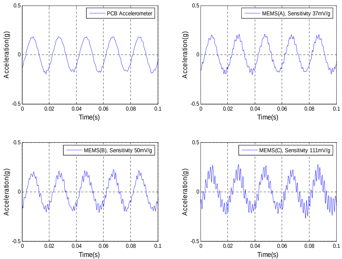
Figure 3 Measured acceleration responses by the MEMS accelerometers and the reference (PCB) accelerometer at 53Hz for the excitation level 0.15g
