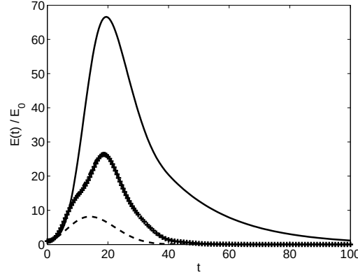
FIG. 5: Linear dynamics of the perturbation energy for the uncontrolled case (—), and closed-loop case actuating with u (— · —), v (---), w (-+). Results for (\alpha = 1, \beta = 1) at Re = 2000 ; in all case, the initial condition is the optimal disturbance for the uncontrolled flow.
