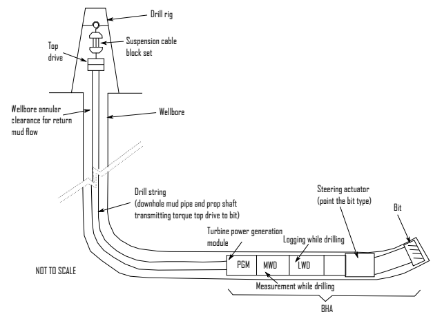
Fig. 1. Schematic of main RSS directional drilling system components
