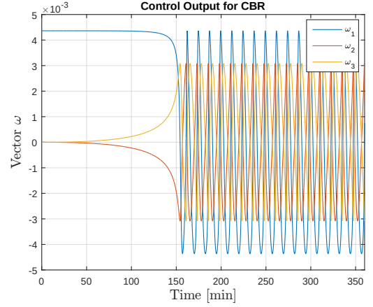
Fig. 5. CBR control output response
