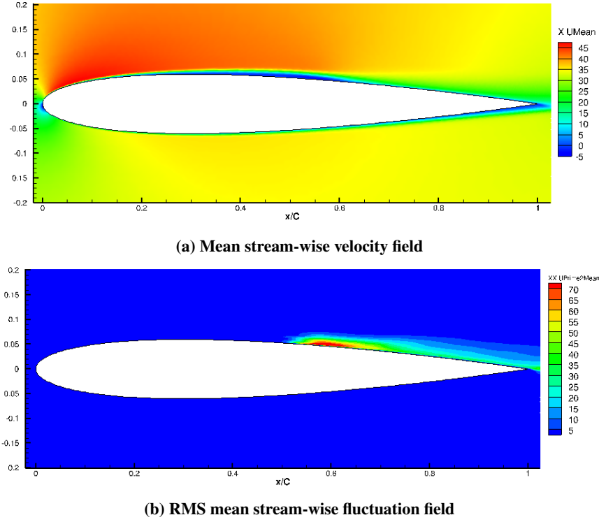
Fig. 7 Time-averaged velocity field, obtained by iLES
