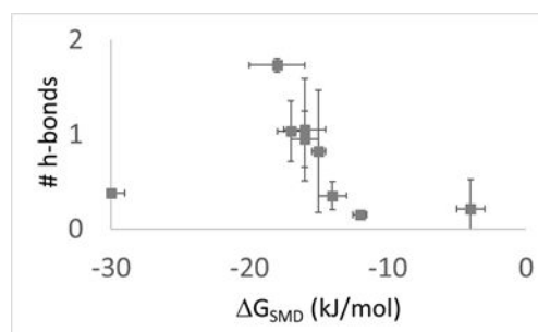
Figure 5. Mean number of hydrogen bonds (H-bonds) between \beta -CD and the ligand molecules v. \Delta G_{\text{SMD}} . Averages are calculated from the bonding states only of the 250ns MD simulations. Standard deviations are calculated from triplicate MD runs.
