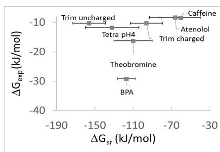
Figure 2. The free binding energies between \beta -CD and ligand molecules calculated by SMD simulations ( \Delta G_{\text{SMD}} ), and the sum of the electrostatic and van der Waals energies between \beta -CD and ligand molecules ( \Delta G_{\text{sr}} ) v. the experimental free binding energies values obtained through previous studied ( \Delta G_{\text{exp}} ) 40-45 .
