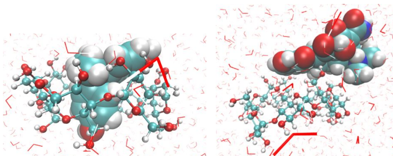
Figure 1. (left) BPA and (right) Tetra. pH8 bound to the \beta -CD cavity.
