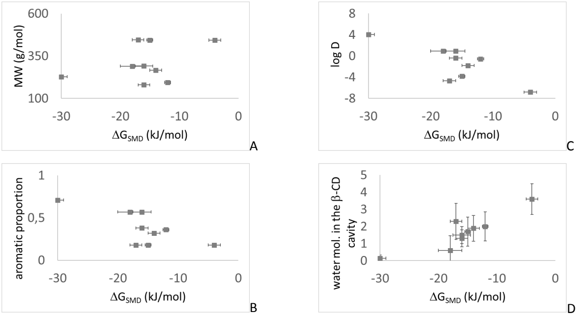
Figure 4. (A) Molar mass (MW), (B) proportion of aromatic cycles, and (C) logD of the different ligand molecules studied v. \Delta G_{SMD} . (D) Mean number of water molecules in the \beta -CD cavity when the different ligand molecules are bound to \beta -CD v. \Delta G_{SMD} . Each average is calculated from the bound states only, of the 250ns MD simulations. Standard deviations are calculated from triplicate MD runs.
