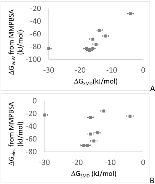
Figure 3. (A) The van der Waals ( \Delta G_{vdw} ) and (B) the electrostatic ( \Delta G_{elec} ) contributions to the enthalpy part of the free binding energy between \beta -CD and ligand molecules v. the free binding energy calculated by SMD analysis ( \Delta G_{SMD} ).
