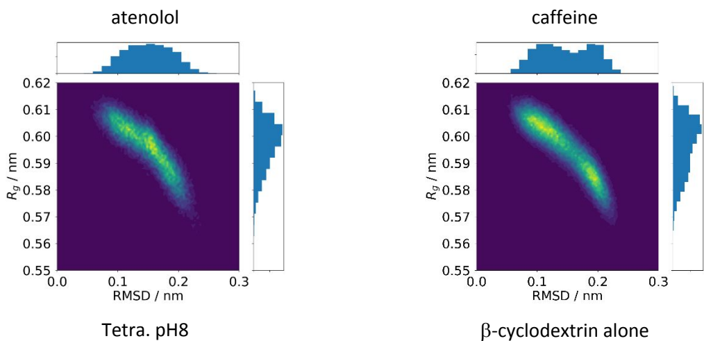
Figure 7. Relative frequency of rmsd (nm) and Rg (nm) for the different complex studied, during bound states, as well as for β-CD alone in water, over the 250ns MD simulation.
